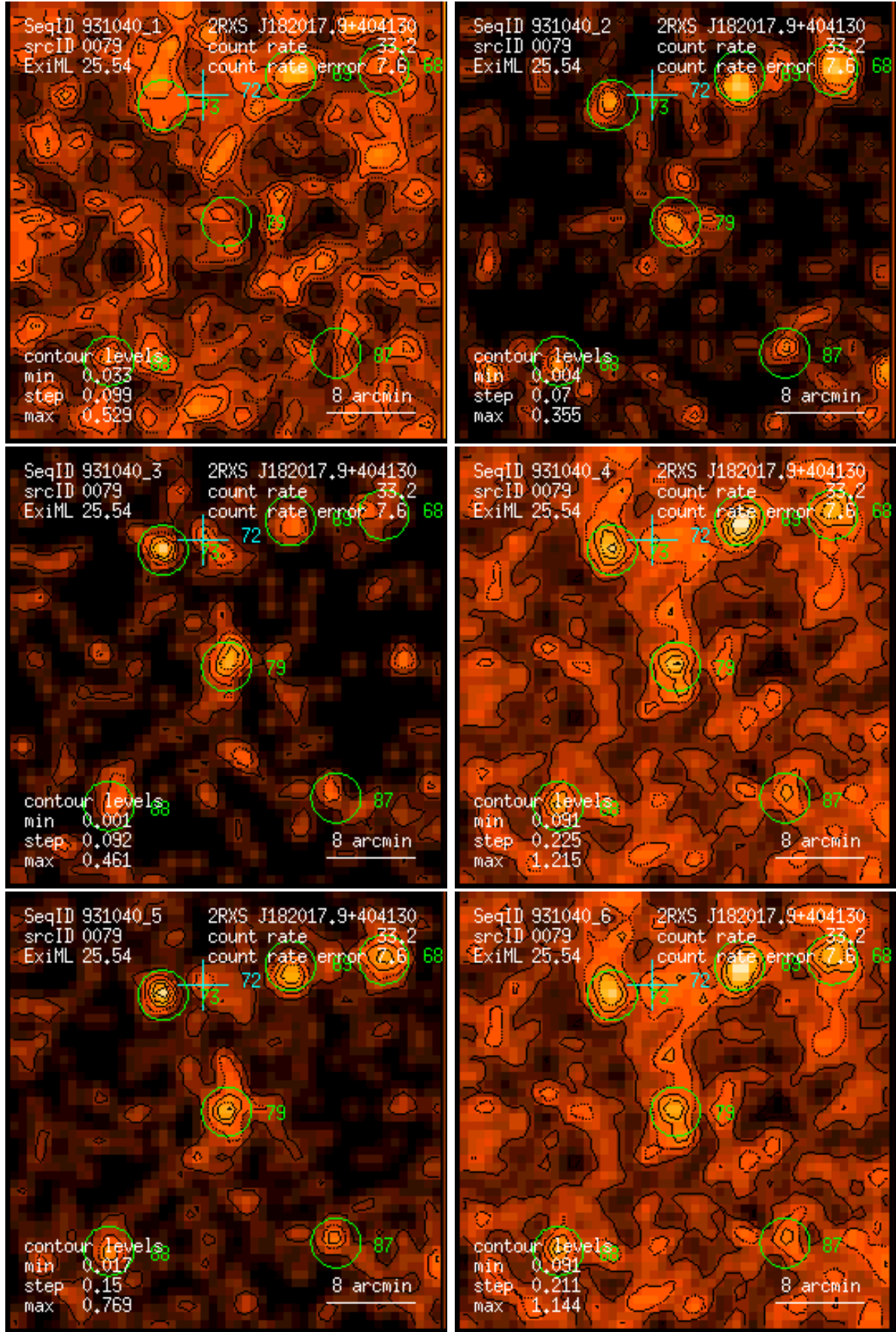
Figure 79: RASS 931040: detection 0079: band rate images, Gaussian filter: (1) PSPC channels 11 – 41, (2) 52 – 90, (3) 91 – 201, (4) 11 – 235, (5) 52 – 201, (6) 11 – 201. Broad band rates in counts/ks. Band rate contour levels in counts/ks/arcmin 2 .
