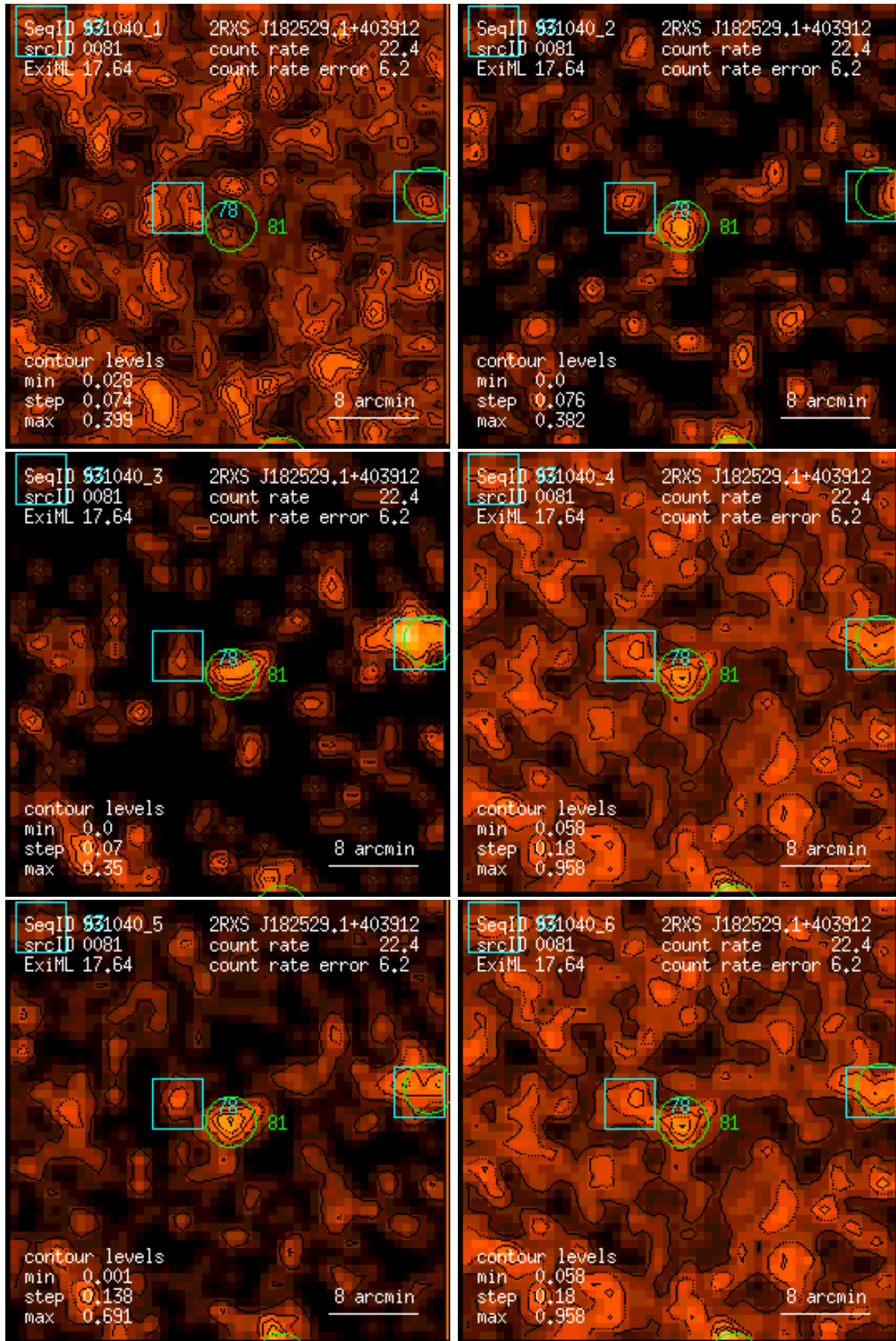
Figure 81: RASS 931040: detection 0081: band rate images, Gaussian filter: (1) PSPC channels 11 – 41, (2) 52 – 90, (3) 91 – 201, (4) 11 – 235, (5) 52 – 201, (6) 11 – 201. Broad band rates in counts/ks. Band rate contour levels in counts/ks/arcmin 2 .
