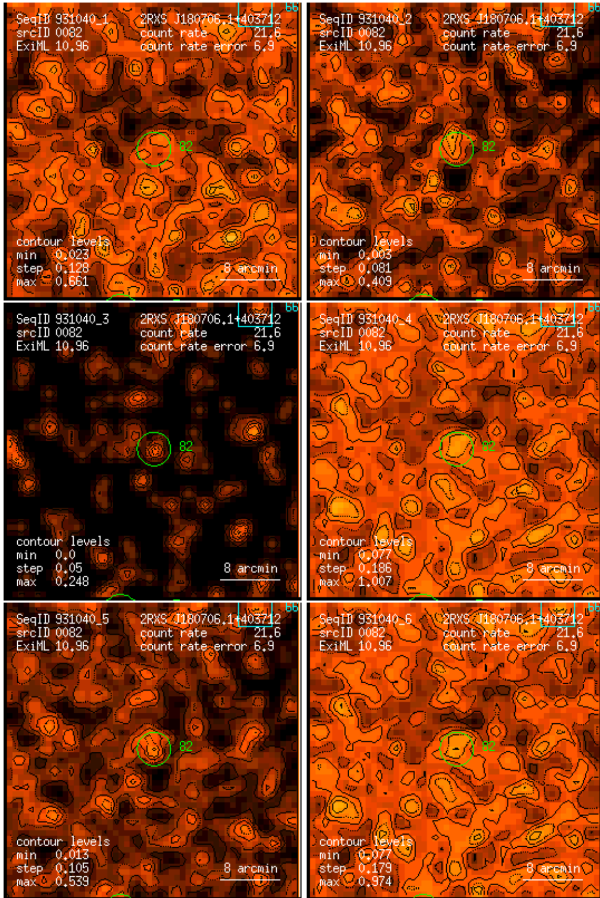
Figure 82: RASS 931040: detection 0082: band rate images, Gaussian filter: (1) PSPC channels 11 – 41, (2) 52 – 90, (3) 91 – 201, (4) 11 – 235, (5) 52 – 201, (6) 11 – 201. Broad band rates in counts/ks. Band rate contour levels in counts/ks/arcmin 2 .
