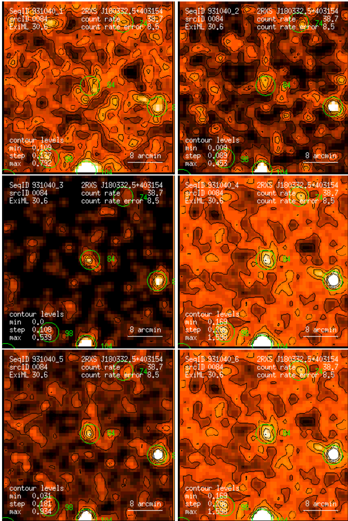
Figure 84: RASS 931040: detection 0084: band rate images, Gaussian filter: (1) PSPC channels 11 – 41, (2) 52 – 90, (3) 91 – 201, (4) 11 – 235, (5) 52 – 201, (6) 11 – 201. Broad band rates in counts/ks. Band rate contour levels in counts/ks/arcmin 2 .
