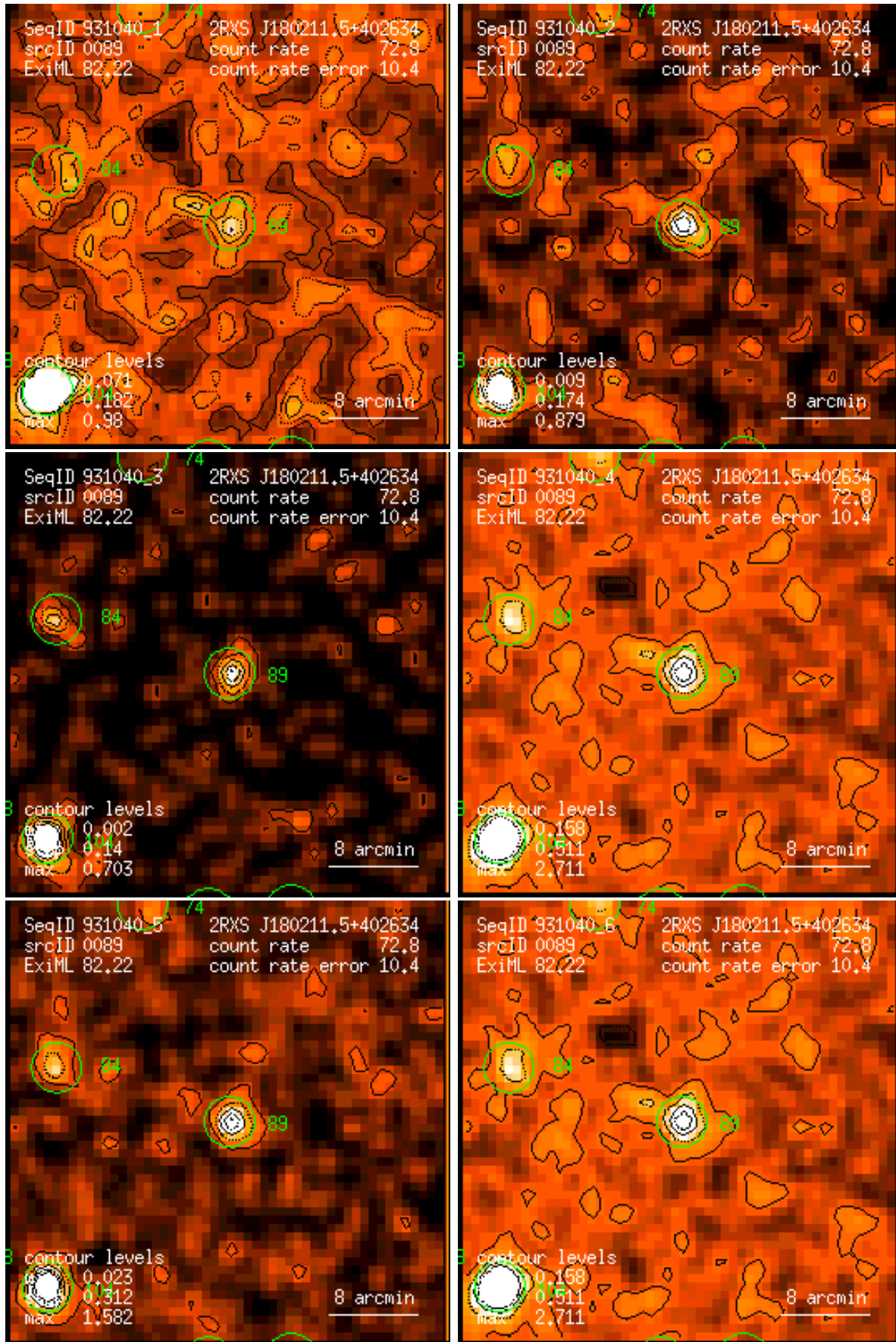
Figure 89: RASS 931040: detection 0089: band rate images, Gaussian filter: (1) PSPC channels 11 – 41, (2) 52 – 90, (3) 91 – 201, (4) 11 – 235, (5) 52 – 201, (6) 11 – 201. Broad band rates in counts/ks. Band rate contour levels in counts/ks/arcmin 2 .
