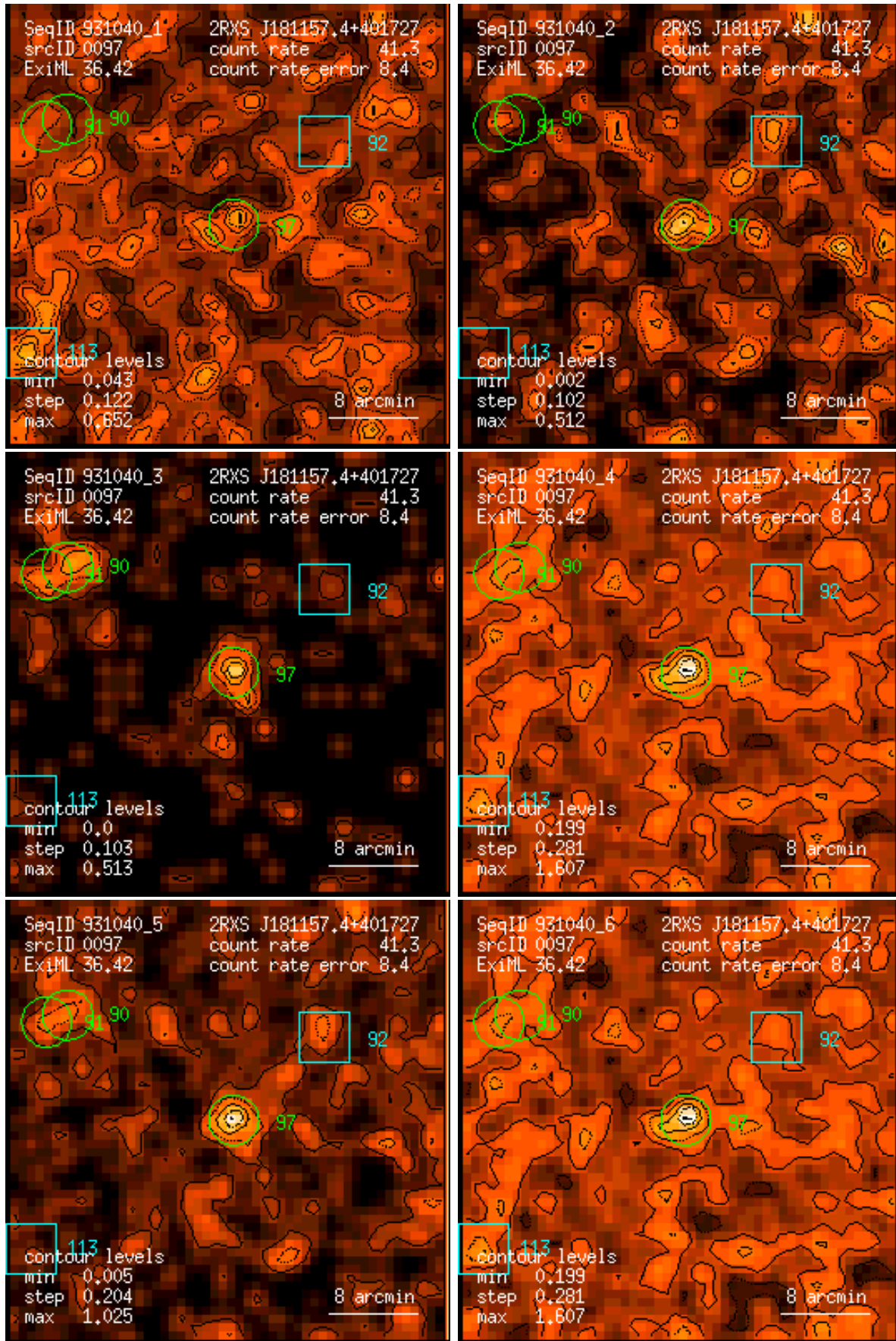
Figure 97: RASS 931040: detection 0097: band rate images, Gaussian filter: (1) PSPC channels 11 – 41, (2) 52 – 90, (3) 91 – 201, (4) 11 – 235, (5) 52 – 201, (6) 11 – 201. Broad band rates in counts/ks. Band rate contour levels in counts/ks/arcmin 2 .
