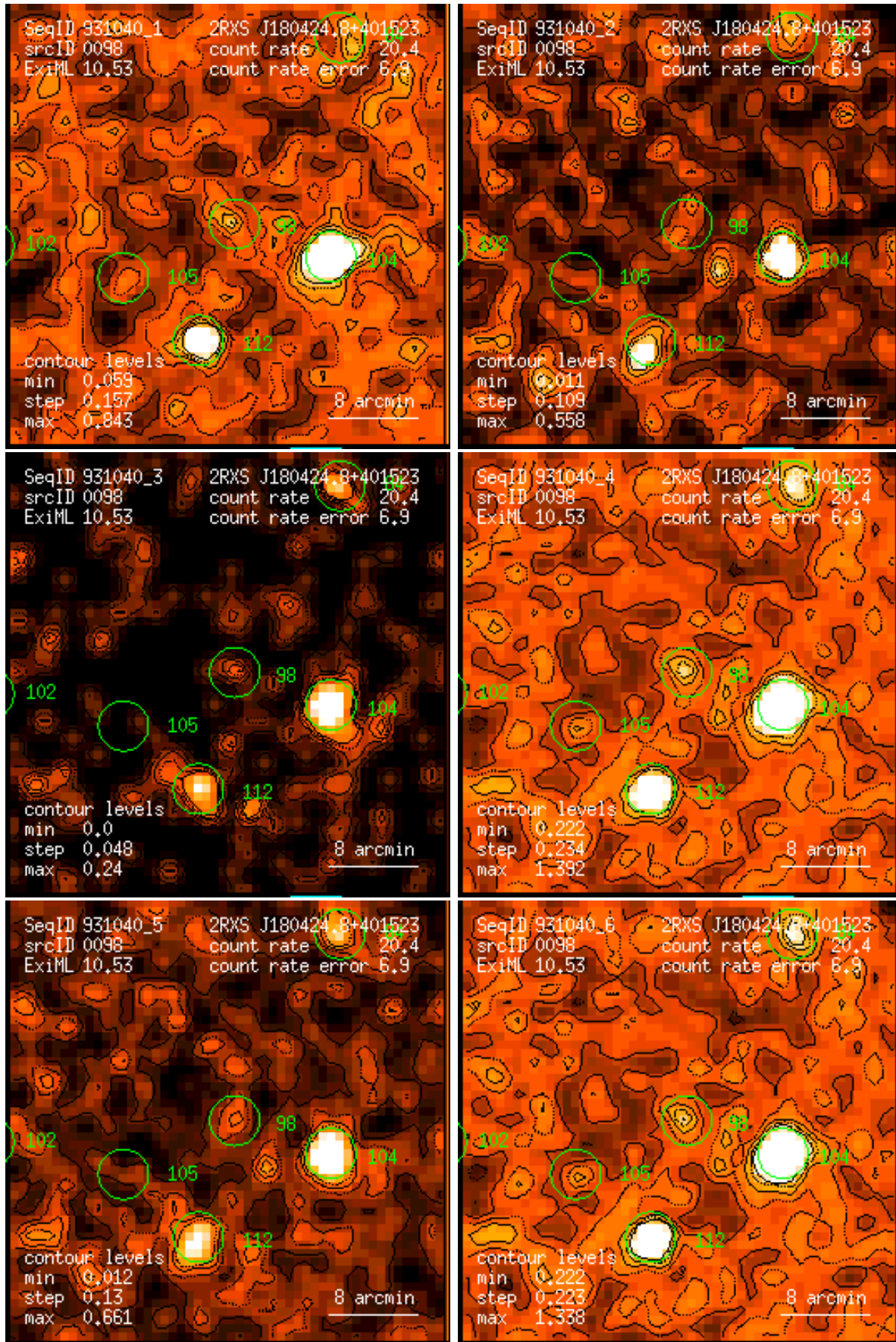
Figure 98: RASS 931040: detection 0098: band rate images, Gaussian filter: (1) PSPC channels 11 – 41, (2) 52 – 90, (3) 91 – 201, (4) 11 – 235, (5) 52 – 201, (6) 11 – 201. Broad band rates in counts/ks. Band rate contour levels in counts/ks/arcmin 2 .
