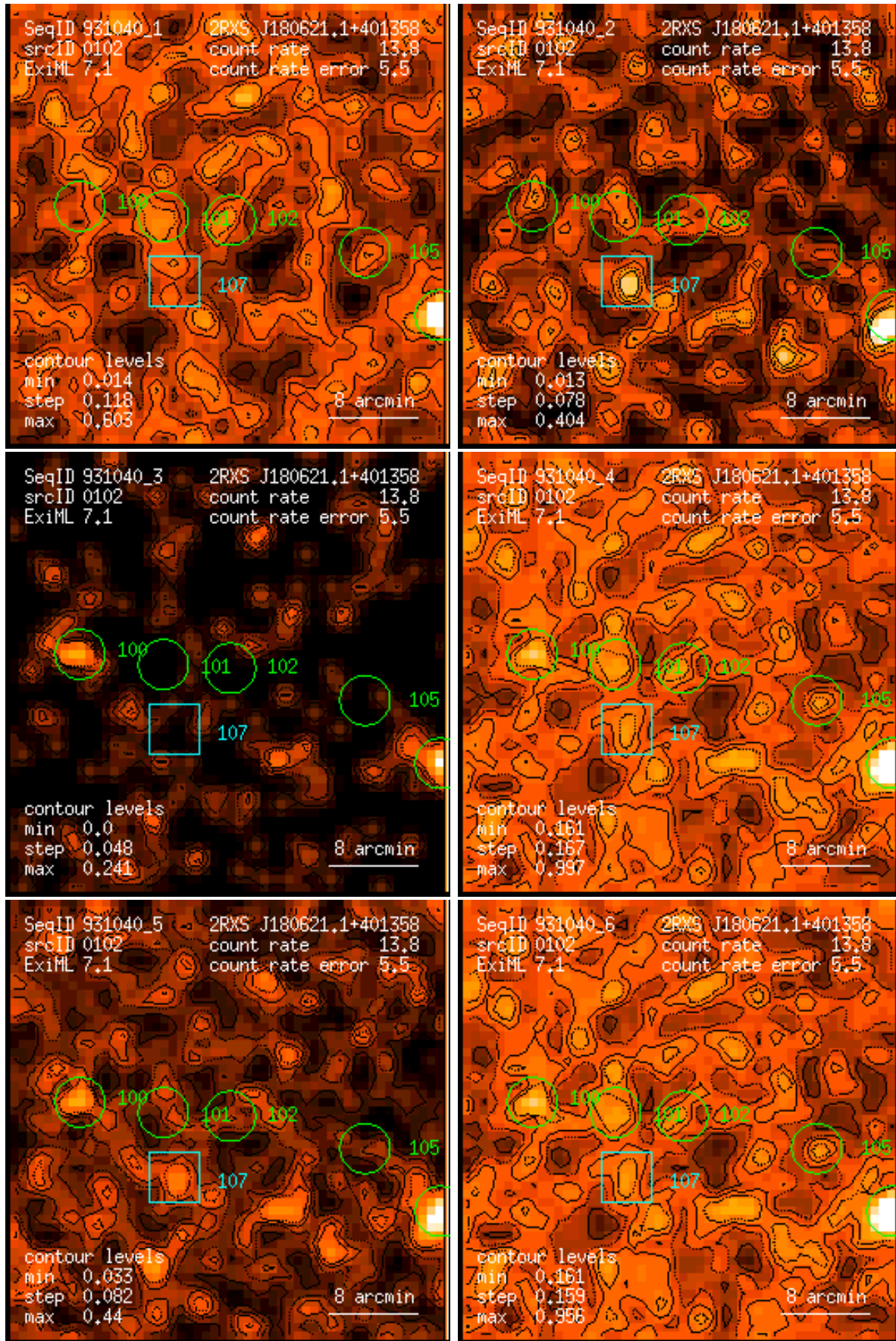
Figure 102: RASS 931040: detection 0102: band rate images, Gaussian filter: (1) PSPC channels 11 – 41, (2) 52 – 90, (3) 91 – 201, (4) 11 – 235, (5) 52 – 201, (6) 11 – 201. Broad band rates in counts/ks. Band rate contour levels in counts/ks/arcmin 2 .
