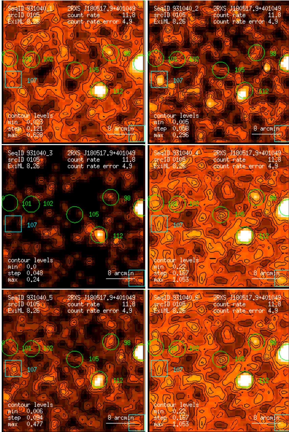
Figure 105: RASS 931040: detection 0105: band rate images, Gaussian filter: (1) PSPC channels 11 – 41, (2) 52 – 90, (3) 91 – 201, (4) 11 – 235, (5) 52 – 201, (6) 11 – 201. Broad band rates in counts/ks. Band rate contour levels in counts/ks/arcmin 2 .
