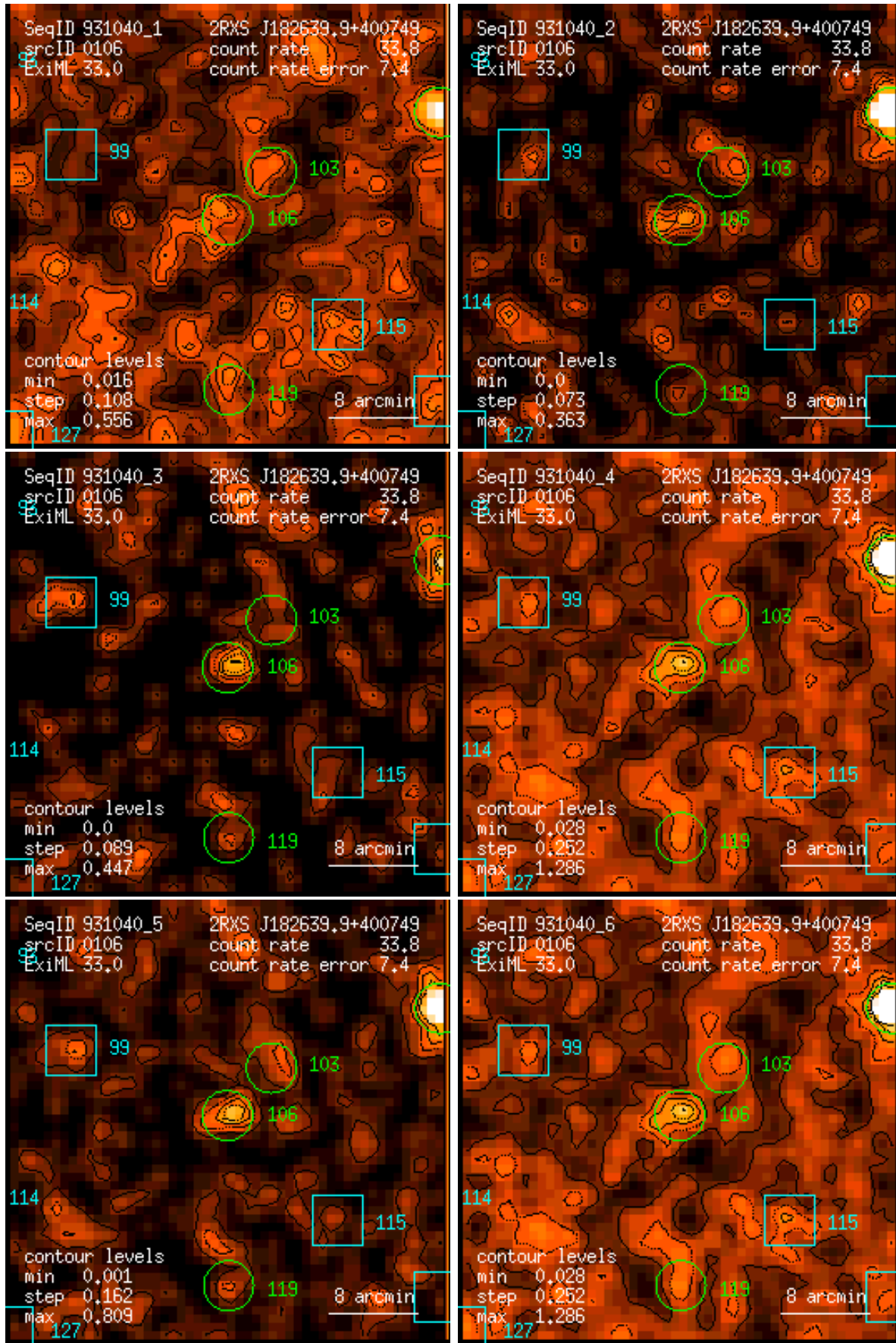
Figure 106: RASS 931040: detection 0106: band rate images, Gaussian filter: (1) PSPC channels 11 – 41, (2) 52 – 90, (3) 91 – 201, (4) 11 – 235, (5) 52 – 201, (6) 11 – 201. Broad band rates in counts/ks. Band rate contour levels in counts/ks/arcmin 2 .
