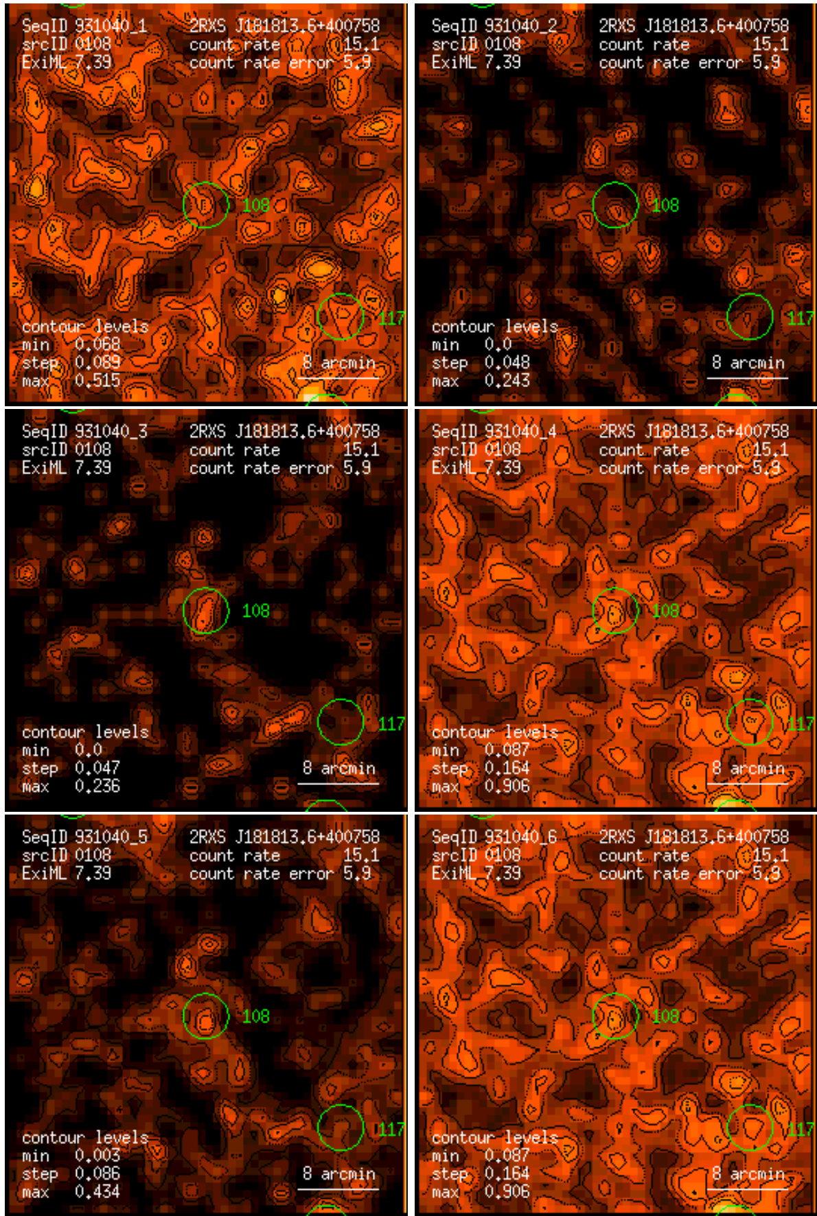
Figure 108: RASS 931040: detection 0108: band rate images, Gaussian filter: (1) PSPC channels 11 – 41, (2) 52 – 90, (3) 91 – 201, (4) 11 – 235, (5) 52 – 201, (6) 11 – 201. Broad band rates in counts/ks. Band rate contour levels in counts/ks/arcmin 2 .
