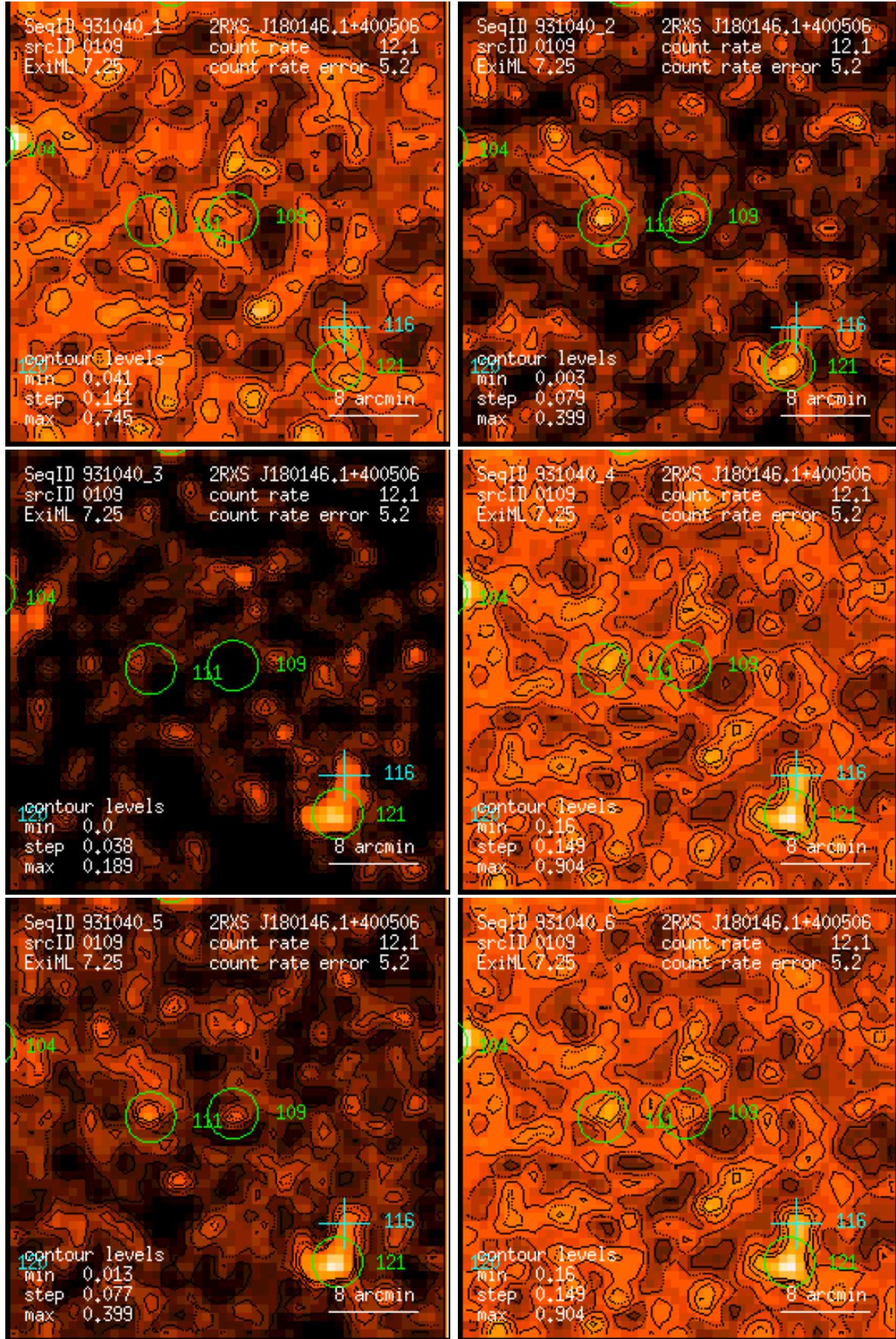
Figure 109: RASS 931040: detection 0109: band rate images, Gaussian filter: (1) PSPC channels 11 – 41, (2) 52 – 90, (3) 91 – 201, (4) 11 – 235, (5) 52 – 201, (6) 11 – 201. Broad band rates in counts/ks. Band rate contour levels in counts/ks/arcmin 2 .
