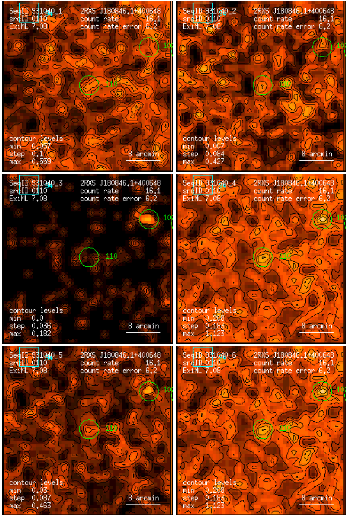
Figure 110: RASS 931040: detection 0110: band rate images, Gaussian filter: (1) PSPC channels 11 – 41, (2) 52 – 90, (3) 91 – 201, (4) 11 – 235, (5) 52 – 201, (6) 11 – 201. Broad band rates in counts/ks. Band rate contour levels in counts/ks/arcmin 2 .
