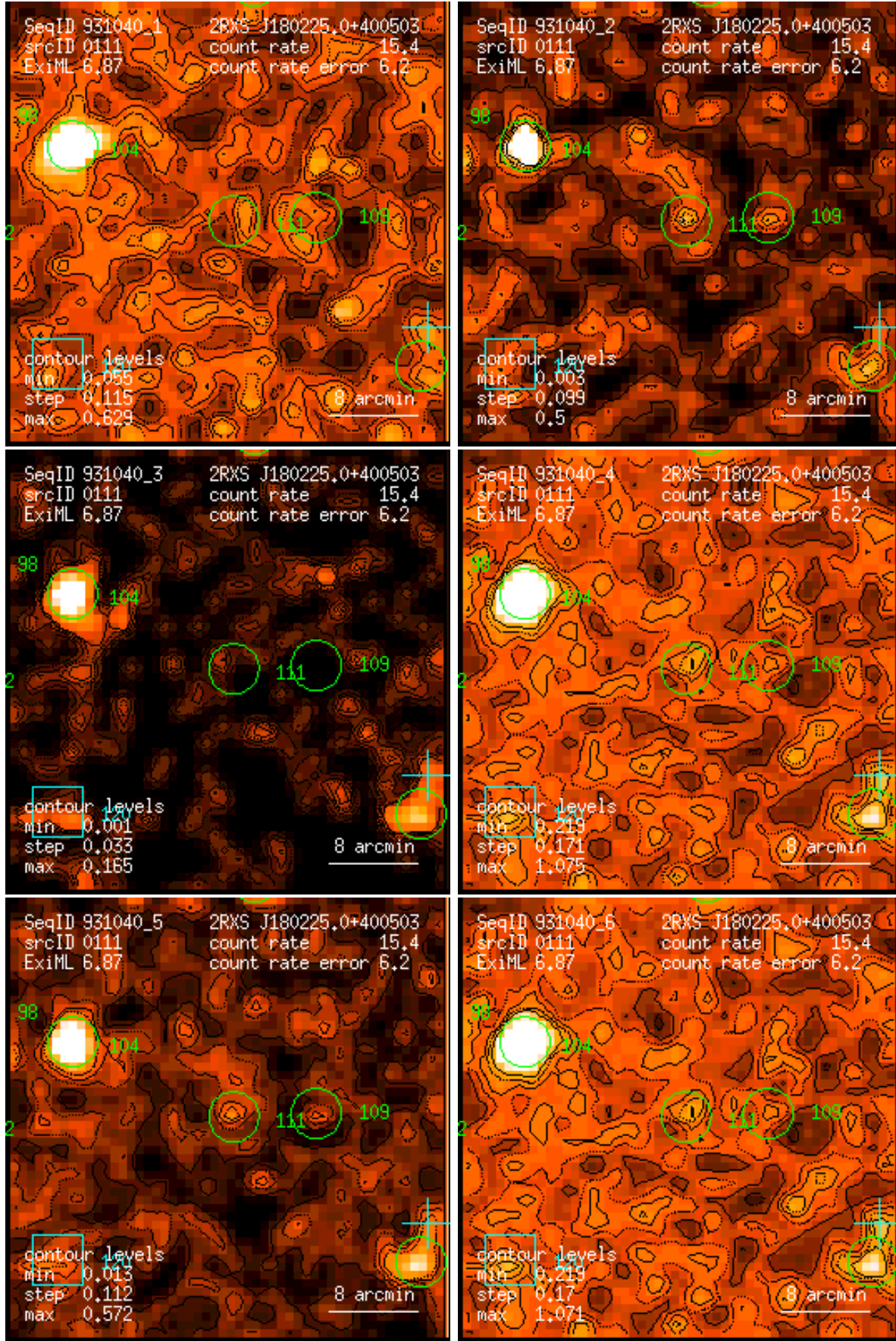
Figure 111: RASS 931040: detection 0111: band rate images, Gaussian filter: (1) PSPC channels 11 – 41, (2) 52 – 90, (3) 91 – 201, (4) 11 – 235, (5) 52 – 201, (6) 11 – 201. Broad band rates in counts/ks. Band rate contour levels in counts/ks/arcmin 2 .
