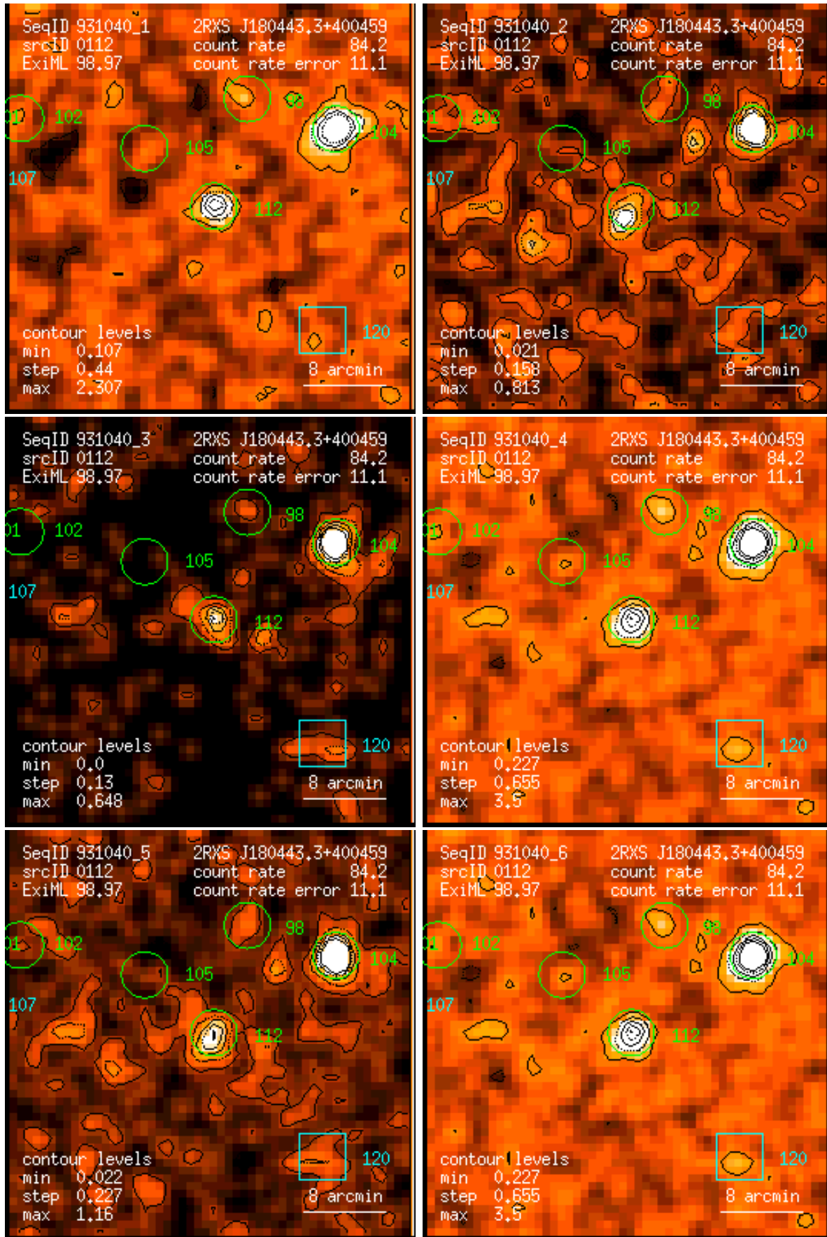
Figure 112: RASS 931040: detection 0112: band rate images, Gaussian filter: (1) PSPC channels 11 – 41, (2) 52 – 90, (3) 91 – 201, (4) 11 – 235, (5) 52 – 201, (6) 11 – 201. Broad band rates in counts/ks. Band rate contour levels in counts/ks/arcmin 2 .
