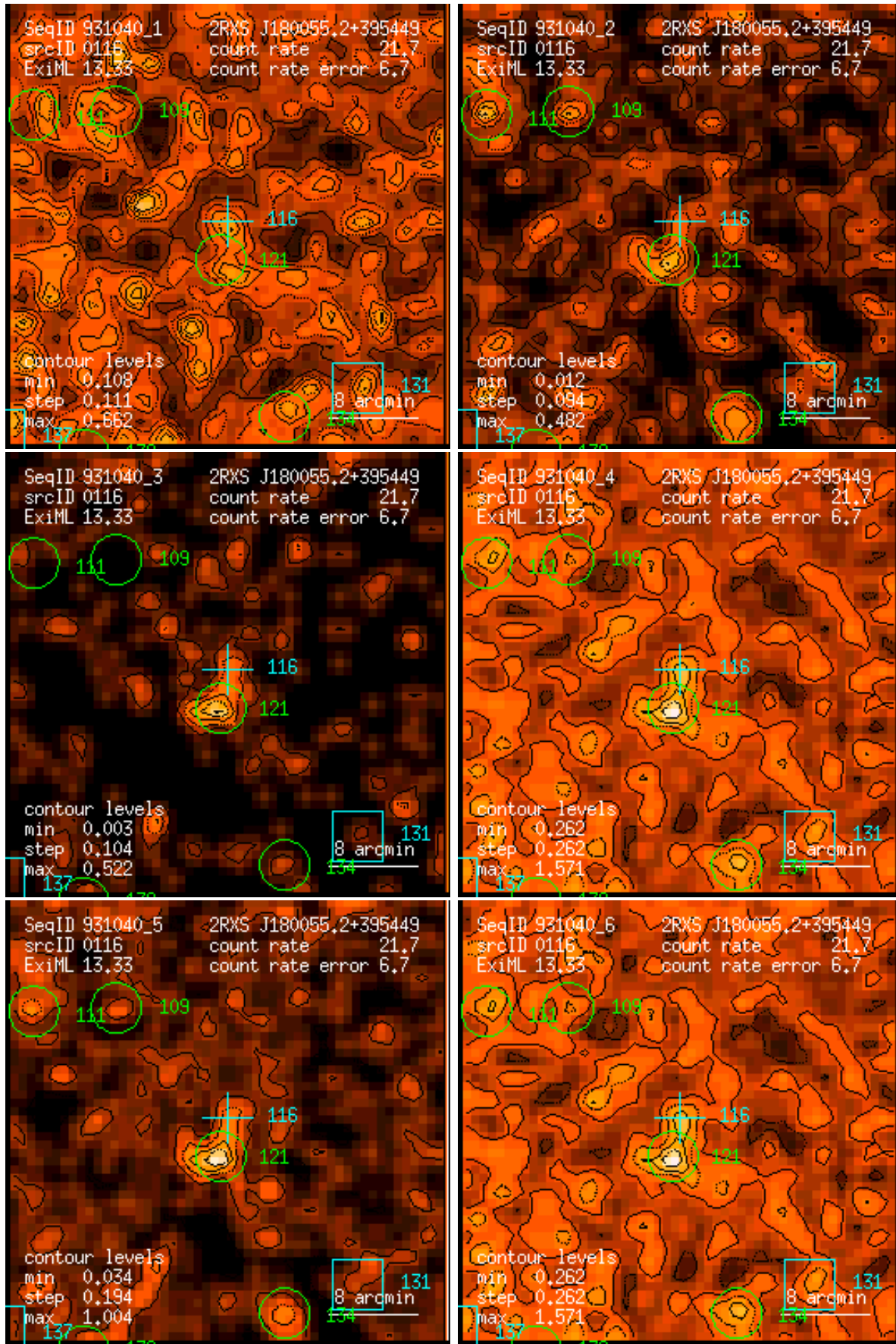
Figure 116: RASS 931040: detection 0116: band rate images, Gaussian filter: (1) PSPC channels 11 – 41, (2) 52 – 90, (3) 91 – 201, (4) 11 – 235, (5) 52 – 201, (6) 11 – 201. Broad band rates in counts/ks. Band rate contour levels in counts/ks/arcmin 2 .
