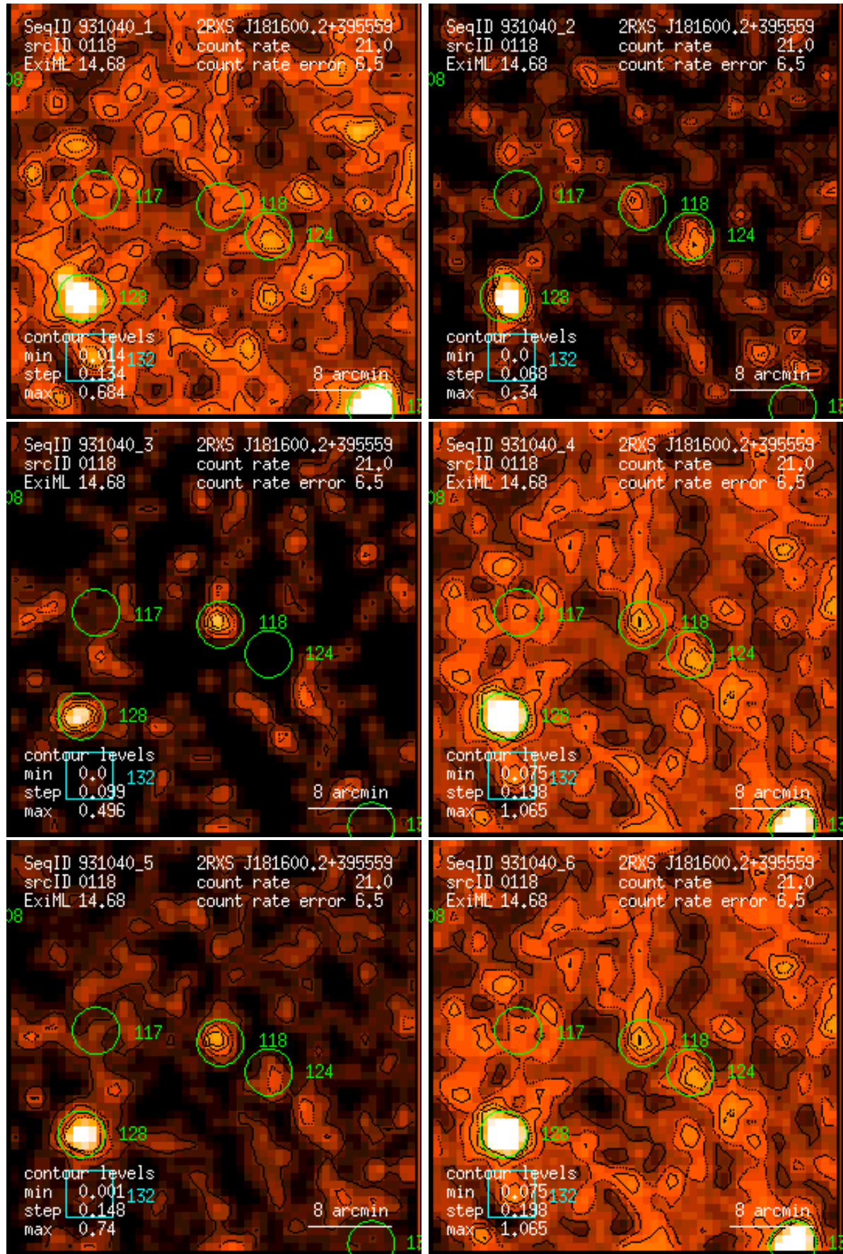
Figure 118: RASS 931040: detection 0118: band rate images, Gaussian filter: (1) PSPC channels 11 – 41, (2) 52 – 90, (3) 91 – 201, (4) 11 – 235, (5) 52 – 201, (6) 11 – 201. Broad band rates in counts/ks. Band rate contour levels in counts/ks/arcmin 2 .
