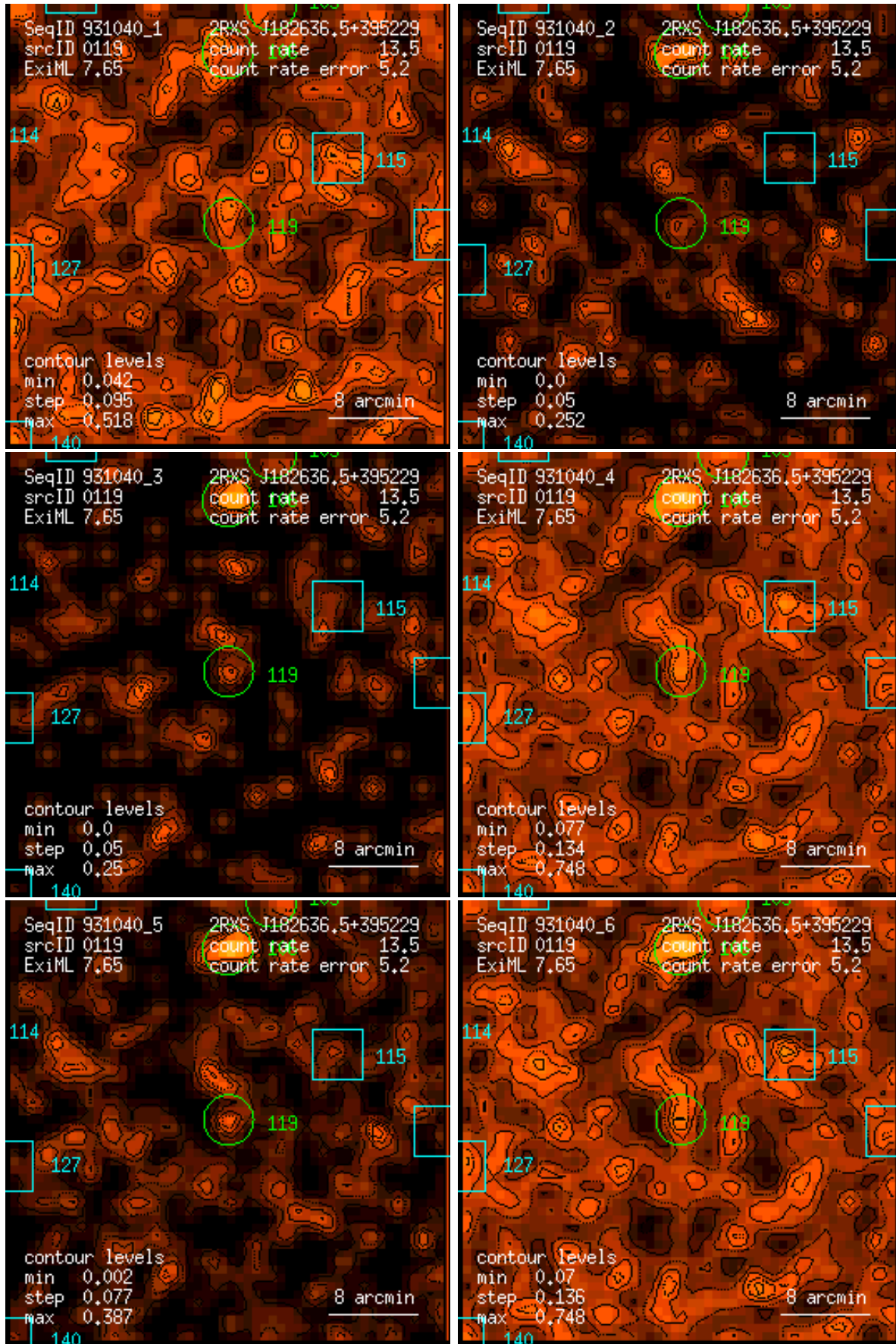
Figure 119: RASS 931040: detection 0119: band rate images, Gaussian filter: (1) PSPC channels 11 – 41, (2) 52 – 90, (3) 91 – 201, (4) 11 – 235, (5) 52 – 201, (6) 11 – 201. Broad band rates in counts/ks. Band rate contour levels in counts/ks/arcmin 2 .
