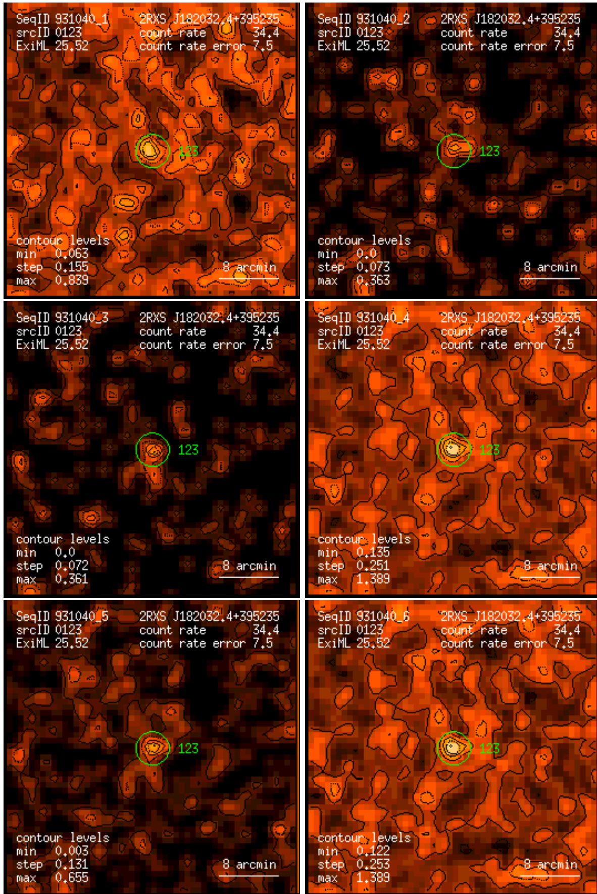
Figure 123: RASS 931040: detection 0123: band rate images, Gaussian filter: (1) PSPC channels 11 – 41, (2) 52 – 90, (3) 91 – 201, (4) 11 – 235, (5) 52 – 201, (6) 11 – 201. Broad band rates in counts/ks. Band rate contour levels in counts/ks/arcmin 2 .
