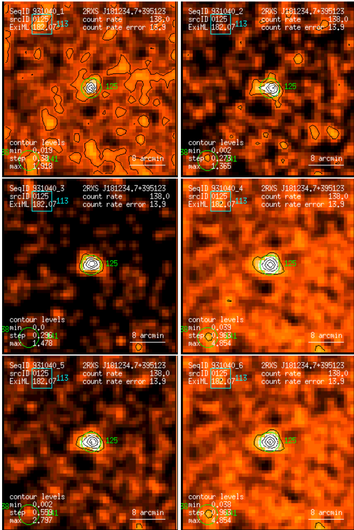
Figure 125: RASS 931040: detection 0125: band rate images, Gaussian filter: (1) PSPC channels 11 – 41, (2) 52 – 90, (3) 91 – 201, (4) 11 – 235, (5) 52 – 201, (6) 11 – 201. Broad band rates in counts/ks. Band rate contour levels in counts/ks/arcmin 2 .
