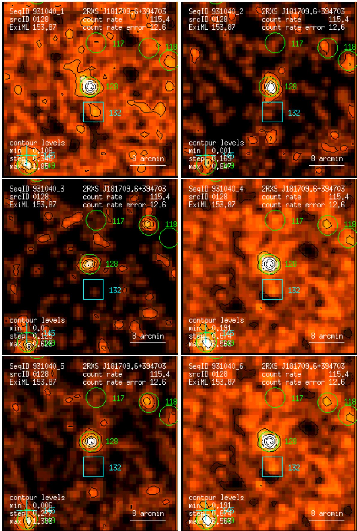
Figure 128: RASS 931040: detection 0128: band rate images, Gaussian filter: (1) PSPC channels 11 – 41, (2) 52 – 90, (3) 91 – 201, (4) 11 – 235, (5) 52 – 201, (6) 11 – 201. Broad band rates in counts/ks. Band rate contour levels in counts/ks/arcmin 2 .
