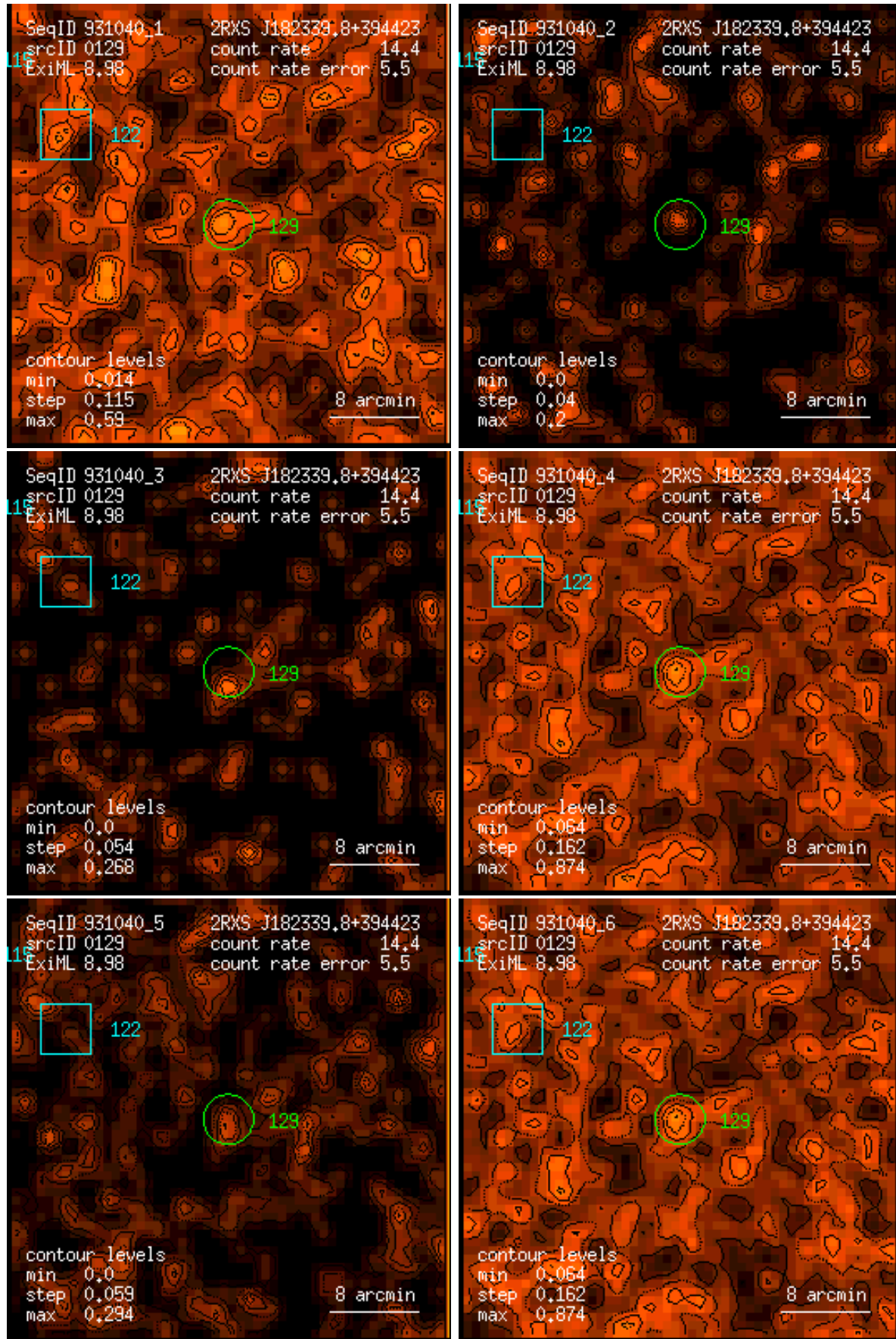
Figure 129: RASS 931040: detection 0129: band rate images, Gaussian filter: (1) PSPC channels 11 – 41, (2) 52 – 90, (3) 91 – 201, (4) 11 – 235, (5) 52 – 201, (6) 11 – 201. Broad band rates in counts/ks. Band rate contour levels in counts/ks/arcmin 2 .
