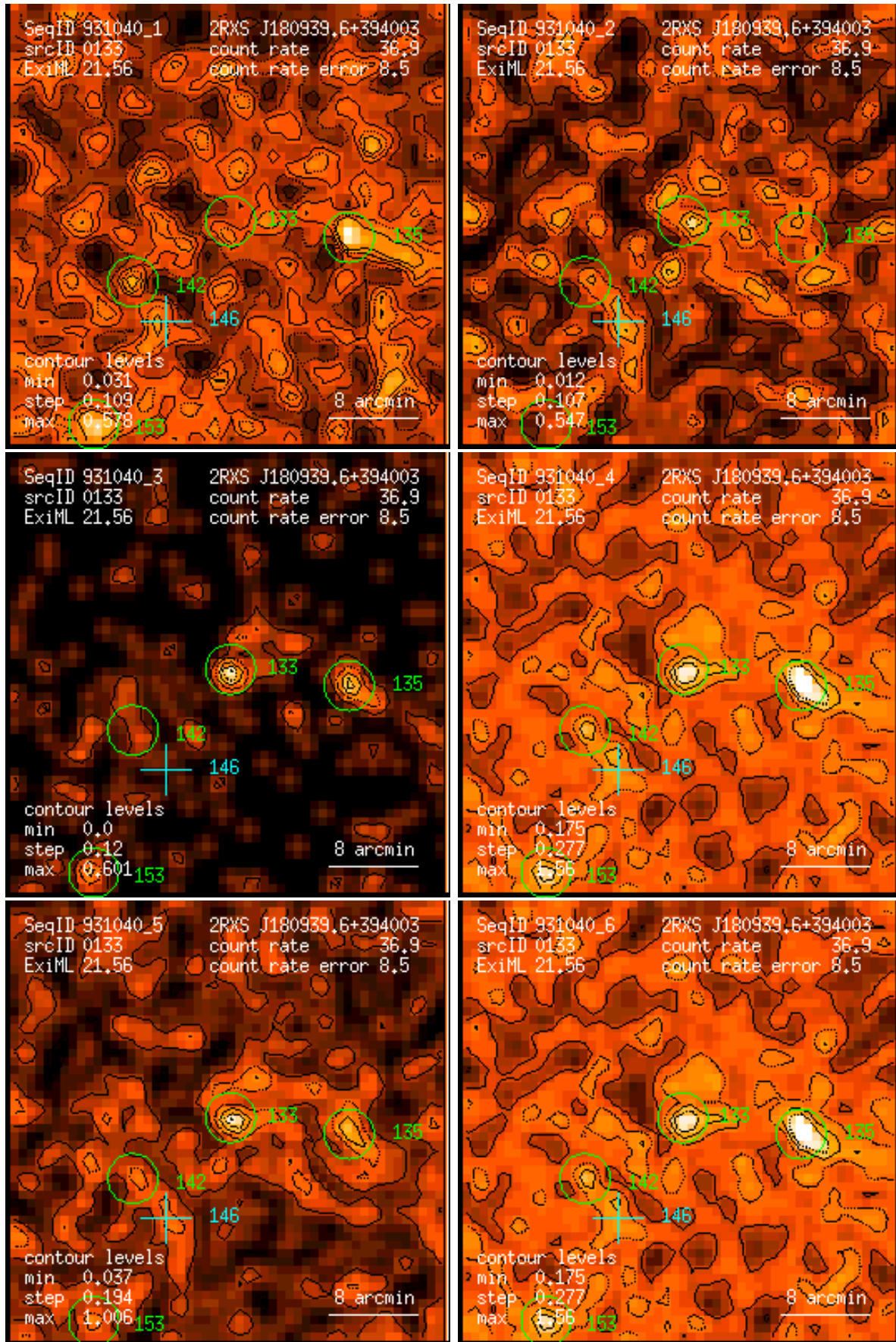
Figure 133: RASS 931040: detection 0133: band rate images, Gaussian filter: (1) PSPC channels 11 – 41, (2) 52 – 90, (3) 91 – 201, (4) 11 – 235, (5) 52 – 201, (6) 11 – 201. Broad band rates in counts/ks. Band rate contour levels in counts/ks/arcmin 2 .
