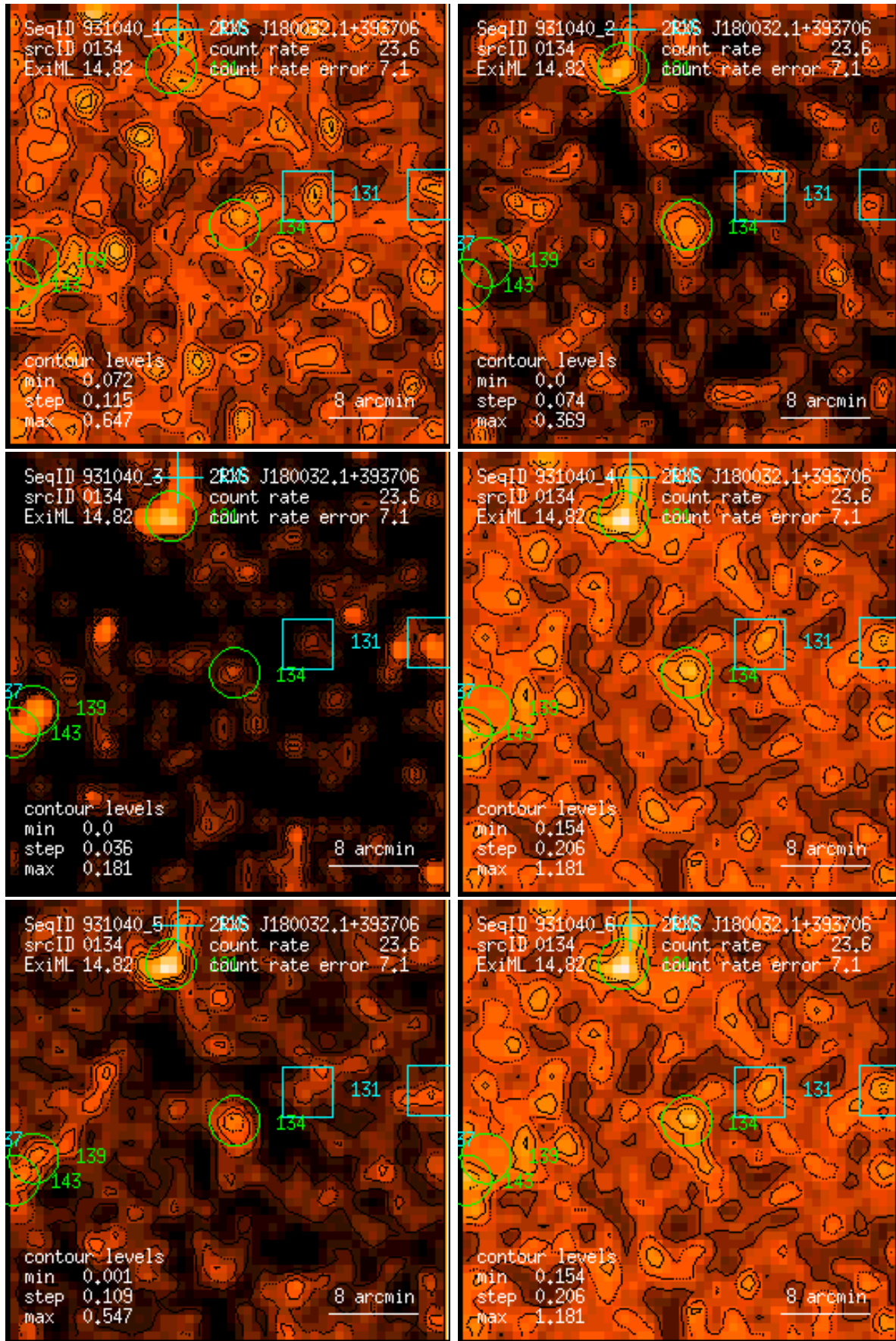
Figure 134: RASS 931040: detection 0134: band rate images, Gaussian filter: (1) PSPC channels 11 – 41, (2) 52 – 90, (3) 91 – 201, (4) 11 – 235, (5) 52 – 201, (6) 11 – 201. Broad band rates in counts/ks. Band rate contour levels in counts/ks/arcmin 2 .
