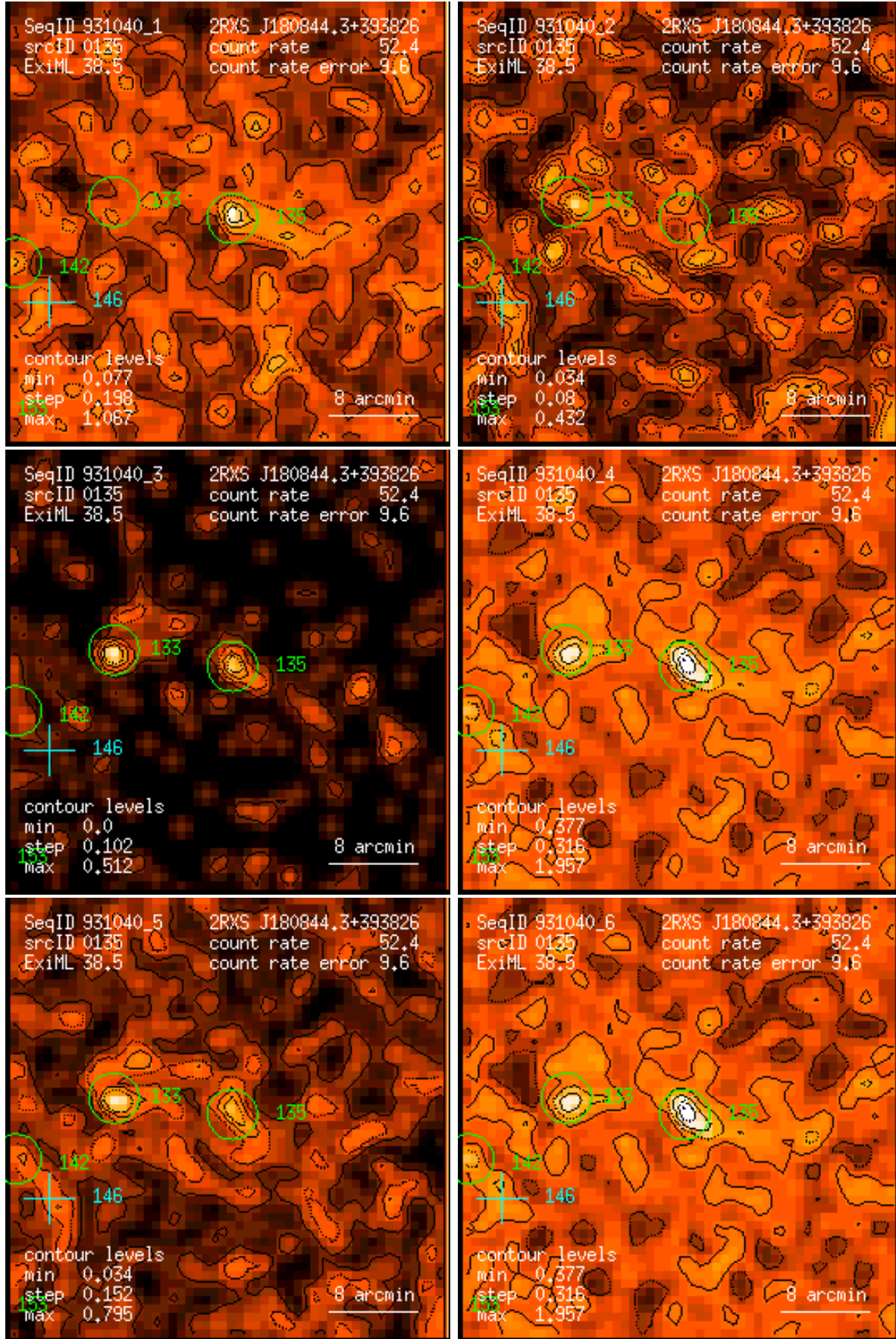
Figure 135: RASS 931040: detection 0135: band rate images, Gaussian filter: (1) PSPC channels 11 – 41, (2) 52 – 90, (3) 91 – 201, (4) 11 – 235, (5) 52 – 201, (6) 11 – 201. Broad band rates in counts/ks. Band rate contour levels in counts/ks/arcmin 2 .
