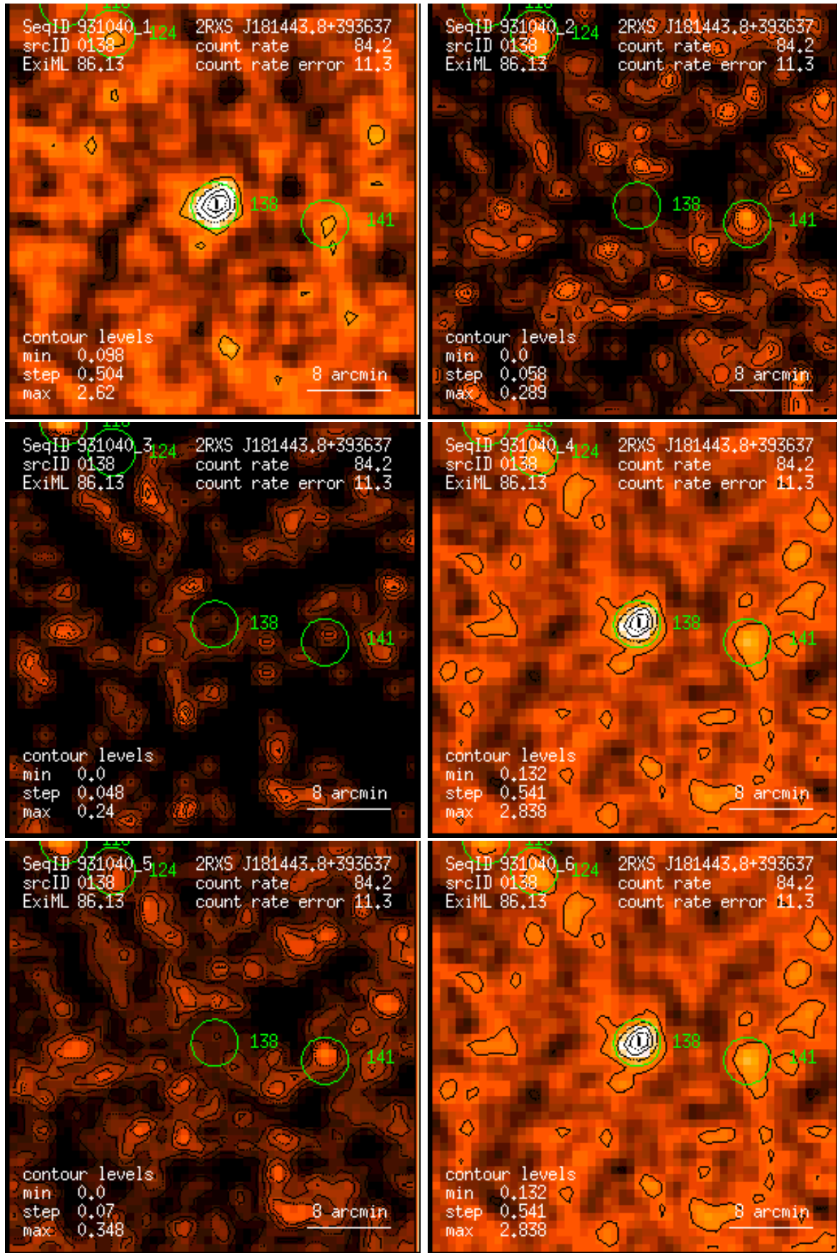
Figure 138: RASS 931040: detection 0138: band rate images, Gaussian filter: (1) PSPC channels 11 – 41, (2) 52 – 90, (3) 91 – 201, (4) 11 – 235, (5) 52 – 201, (6) 11 – 201. Broad band rates in counts/ks. Band rate contour levels in counts/ks/arcmin 2 .
