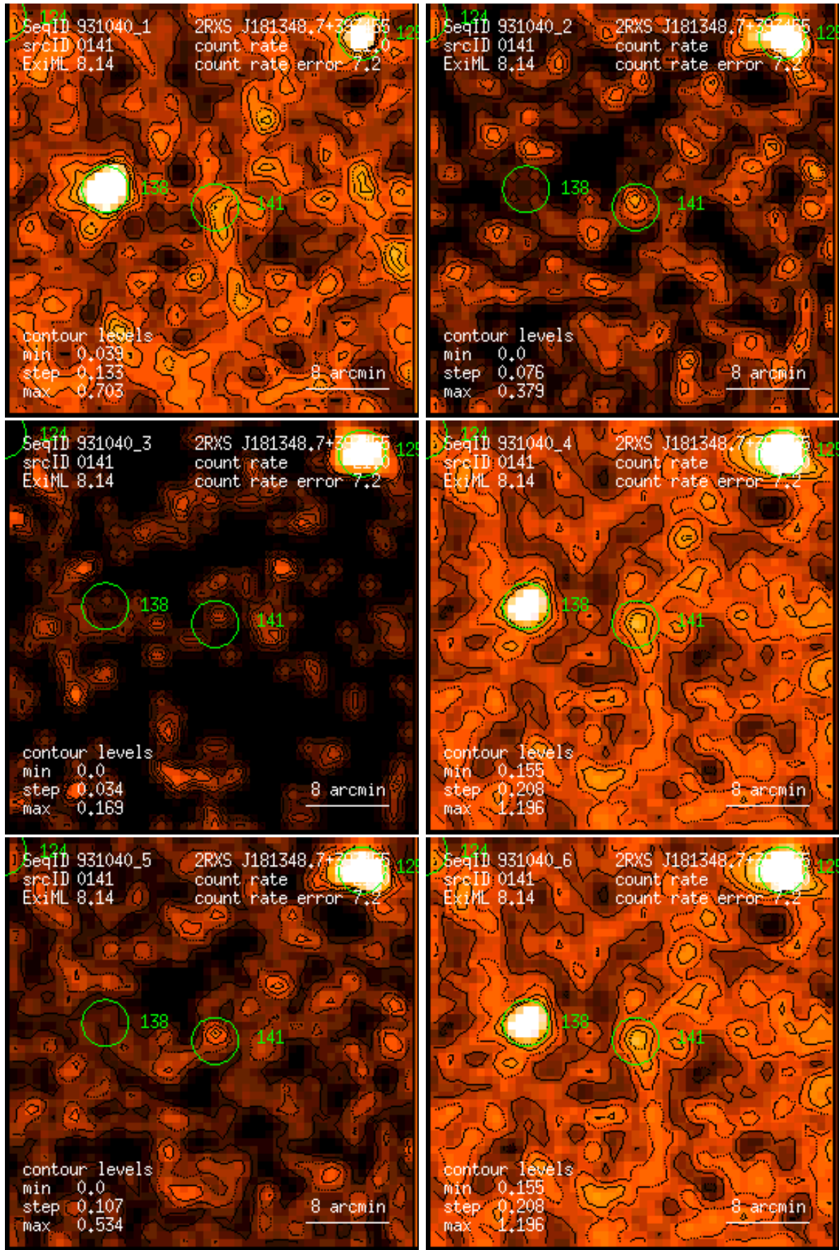
Figure 141: RASS 931040: detection 0141: band rate images, Gaussian filter: (1) PSPC channels 11 – 41, (2) 52 – 90, (3) 91 – 201, (4) 11 – 235, (5) 52 – 201, (6) 11 – 201. Broad band rates in counts/ks. Band rate contour levels in counts/ks/arcmin 2 .
