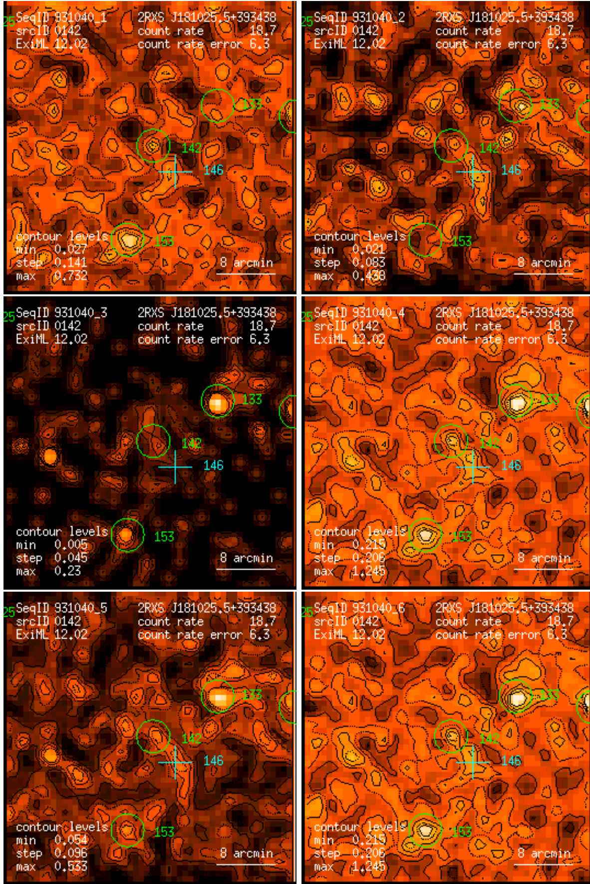
Figure 142: RASS 931040: detection 0142: band rate images, Gaussian filter: (1) PSPC channels 11 – 41, (2) 52 – 90, (3) 91 – 201, (4) 11 – 235, (5) 52 – 201, (6) 11 – 201. Broad band rates in counts/ks. Band rate contour levels in counts/ks/arcmin 2 .
