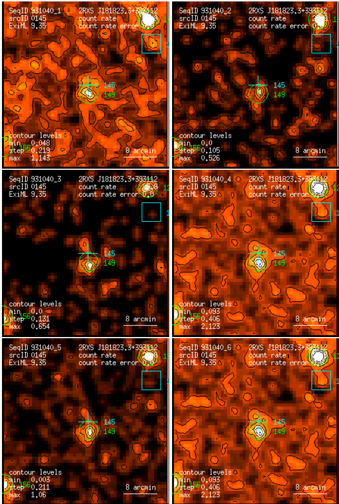
Figure 145: RASS 931040: detection 0145: band rate images, Gaussian filter: (1) PSPC channels 11 – 41, (2) 52 – 90, (3) 91 – 201, (4) 11 – 235, (5) 52 – 201, (6) 11 – 201. Broad band rates in counts/ks. Band rate contour levels in counts/ks/arcmin 2 .
