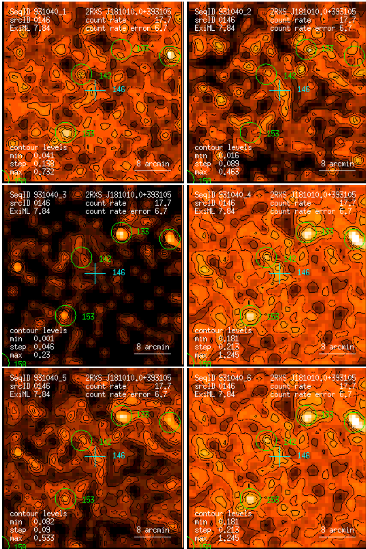
Figure 146: RASS 931040: detection 0146: band rate images, Gaussian filter: (1) PSPC channels 11 – 41, (2) 52 – 90, (3) 91 – 201, (4) 11 – 235, (5) 52 – 201, (6) 11 – 201. Broad band rates in counts/ks. Band rate contour levels in counts/ks/arcmin 2 .
