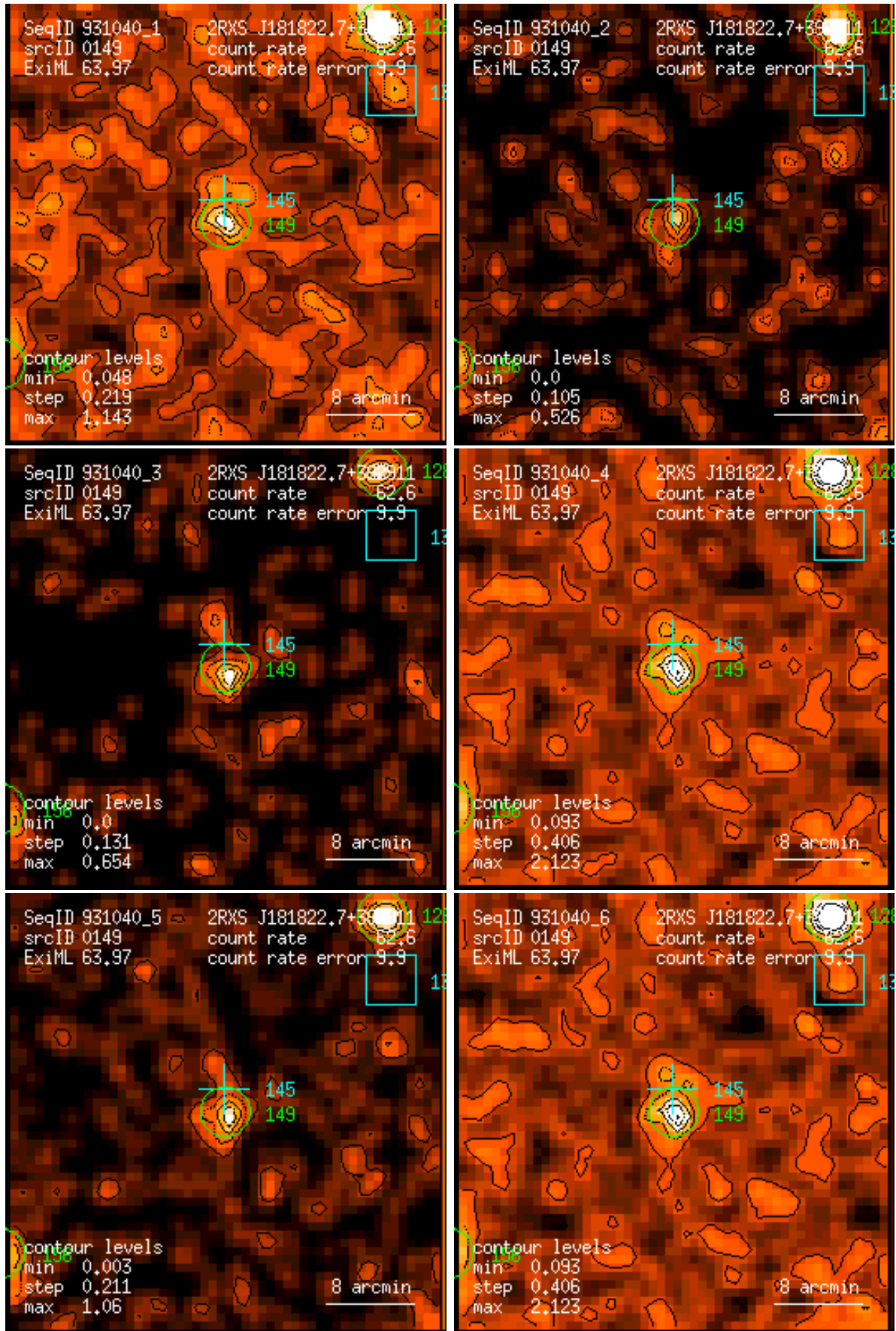
Figure 149: RASS 931040: detection 0149: band rate images, Gaussian filter: (1) PSPC channels 11 – 41, (2) 52 – 90, (3) 91 – 201, (4) 11 – 235, (5) 52 – 201, (6) 11 – 201. Broad band rates in counts/ks. Band rate contour levels in counts/ks/arcmin 2 .
