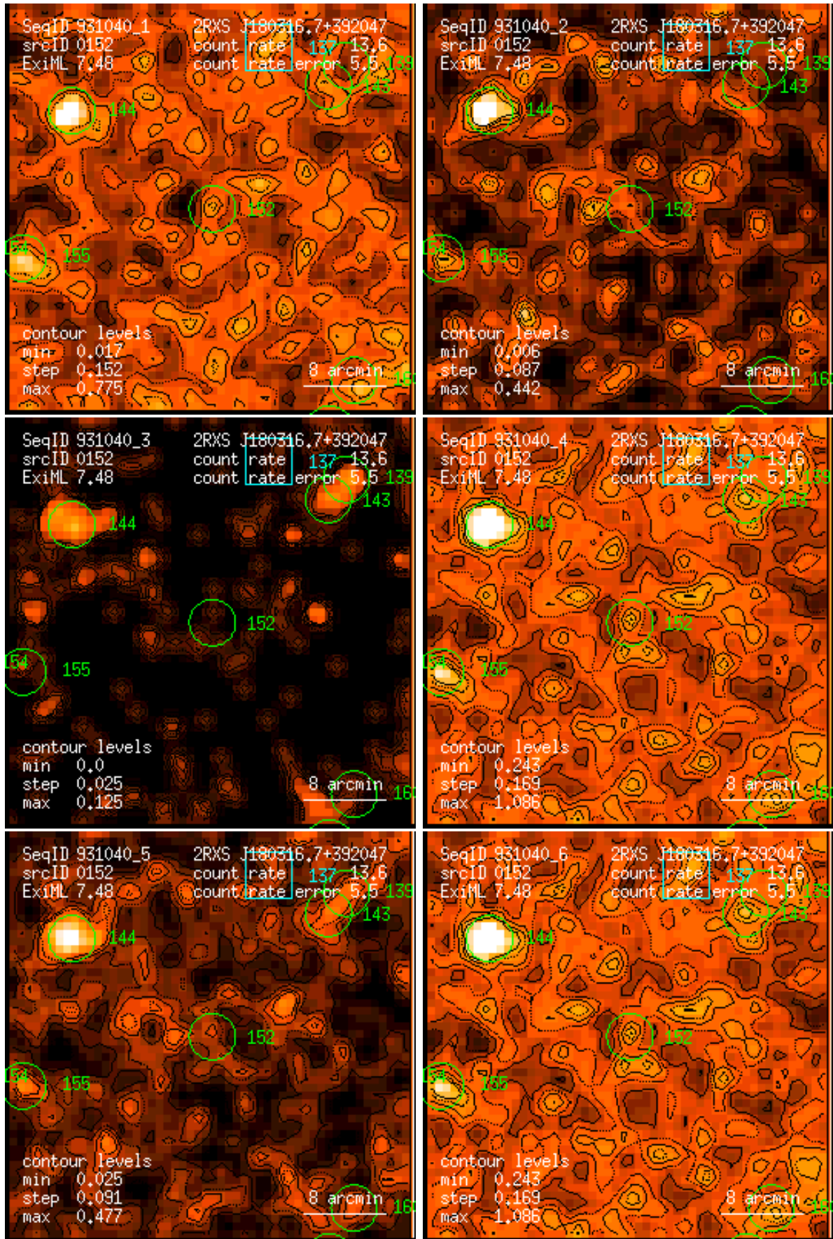
Figure 152: RASS 931040: detection 0152: band rate images, Gaussian filter: (1) PSPC channels 11 – 41, (2) 52 – 90, (3) 91 – 201, (4) 11 – 235, (5) 52 – 201, (6) 11 – 201. Broad band rates in counts/ks. Band rate contour levels in counts/ks/arcmin 2 .
