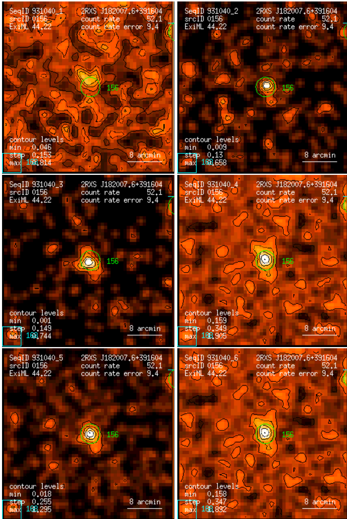
Figure 156: RASS 931040: detection 0156: band rate images, Gaussian filter: (1) PSPC channels 11 – 41, (2) 52 – 90, (3) 91 – 201, (4) 11 – 235, (5) 52 – 201, (6) 11 – 201. Broad band rates in counts/ks. Band rate contour levels in counts/ks/arcmin 2 .
