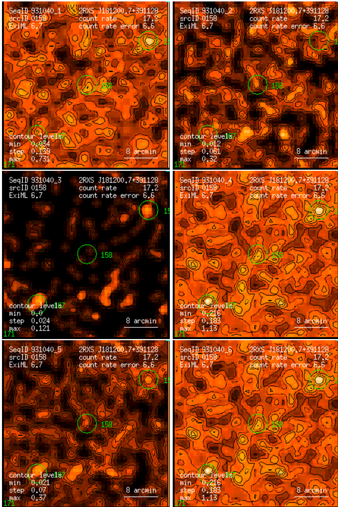
Figure 158: RASS 931040: detection 0158: band rate images, Gaussian filter: (1) PSPC channels 11 – 41, (2) 52 – 90, (3) 91 – 201, (4) 11 – 235, (5) 52 – 201, (6) 11 – 201. Broad band rates in counts/ks. Band rate contour levels in counts/ks/arcmin 2 .
