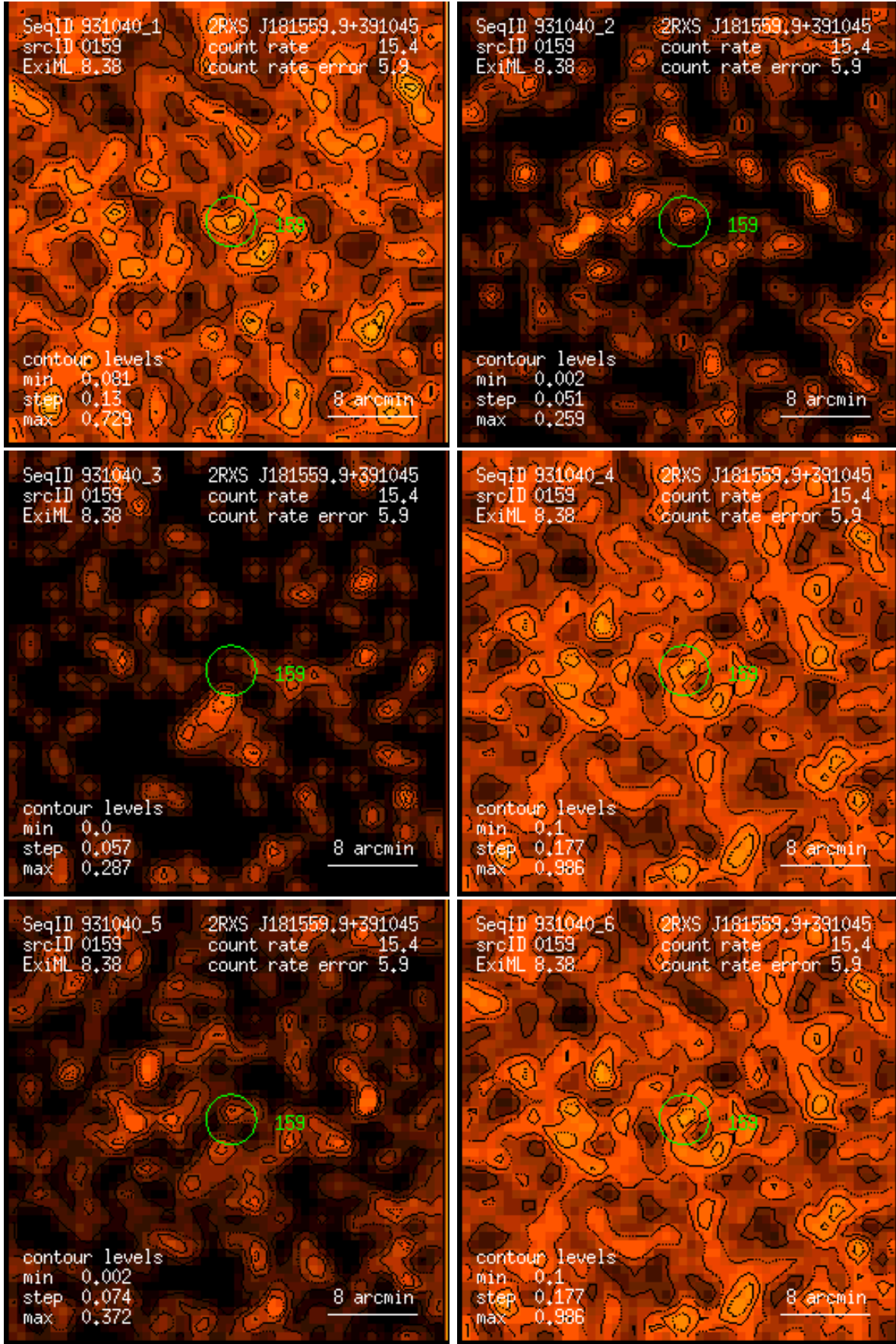
Figure 159: RASS 931040: detection 0159: band rate images, Gaussian filter: (1) PSPC channels 11 – 41, (2) 52 – 90, (3) 91 – 201, (4) 11 – 235, (5) 52 – 201, (6) 11 – 201. Broad band rates in counts/ks. Band rate contour levels in counts/ks/arcmin 2 .
