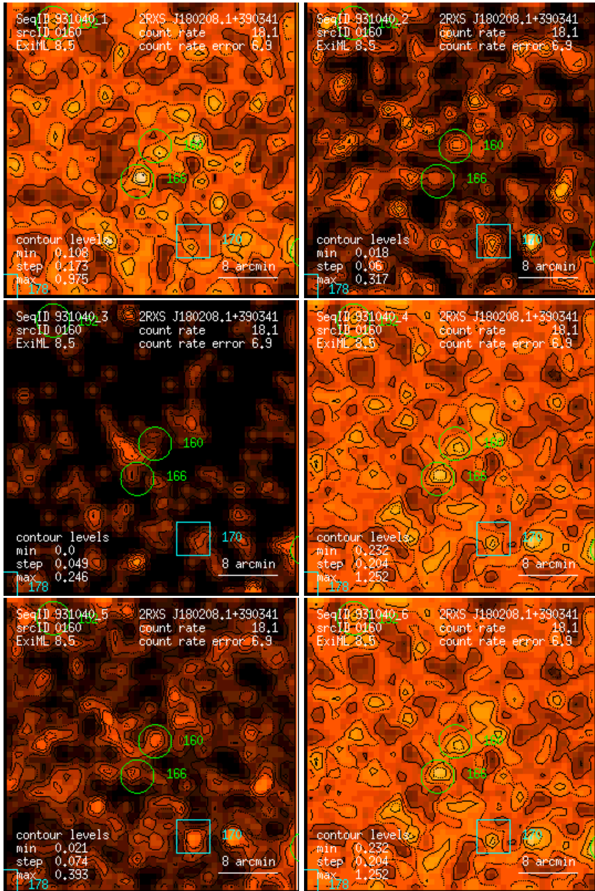
Figure 160: RASS 931040: detection 0160: band rate images, Gaussian filter: (1) PSPC channels 11 – 41, (2) 52 – 90, (3) 91 – 201, (4) 11 – 235, (5) 52 – 201, (6) 11 – 201. Broad band rates in counts/ks. Band rate contour levels in counts/ks/arcmin 2 .
