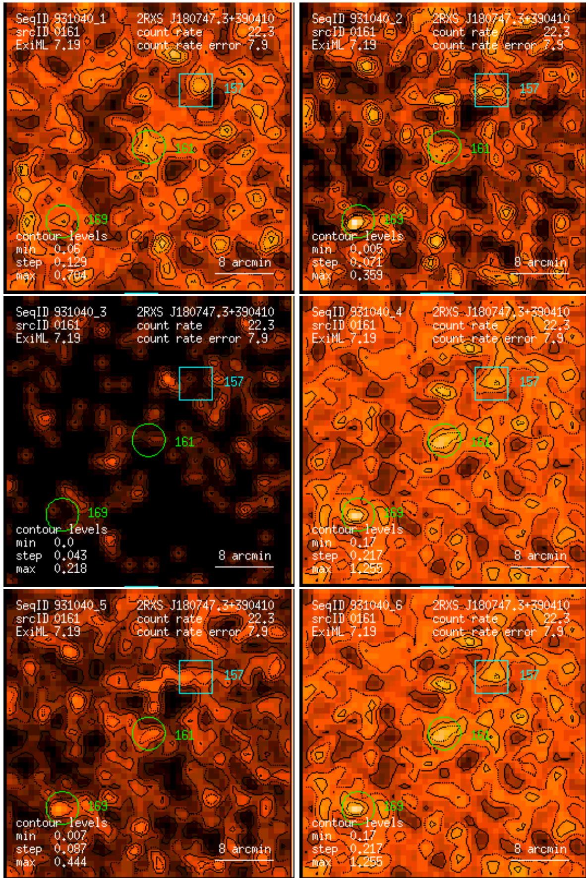
Figure 161: RASS 931040: detection 0161: band rate images, Gaussian filter: (1) PSPC channels 11 – 41, (2) 52 – 90, (3) 91 – 201, (4) 11 – 235, (5) 52 – 201, (6) 11 – 201. Broad band rates in counts/ks. Band rate contour levels in counts/ks/arcmin 2 .
