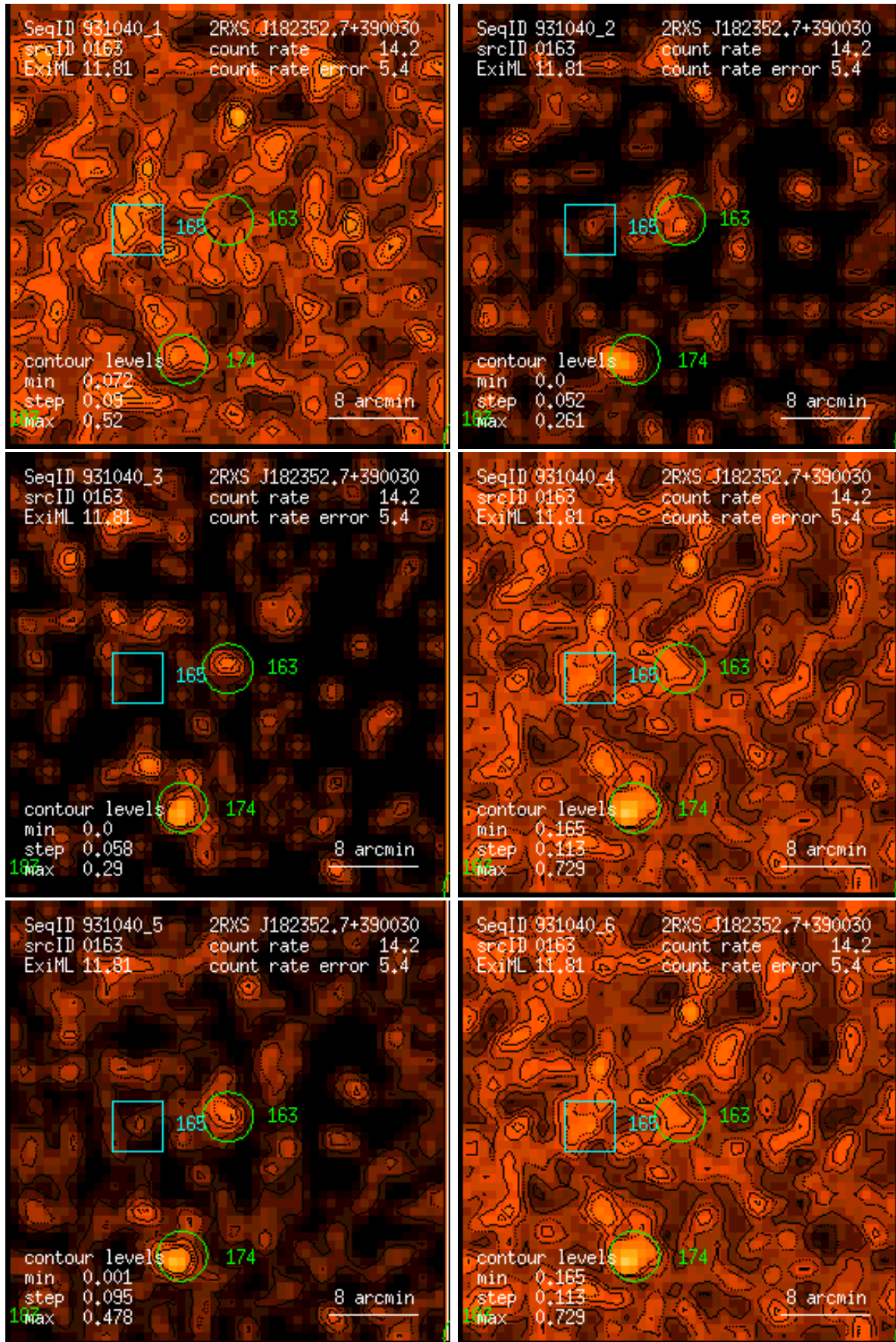
Figure 163: RASS 931040: detection 0163: band rate images, Gaussian filter: (1) PSPC channels 11 – 41, (2) 52 – 90, (3) 91 – 201, (4) 11 – 235, (5) 52 – 201, (6) 11 – 201. Broad band rates in counts/ks. Band rate contour levels in counts/ks/arcmin 2 .
