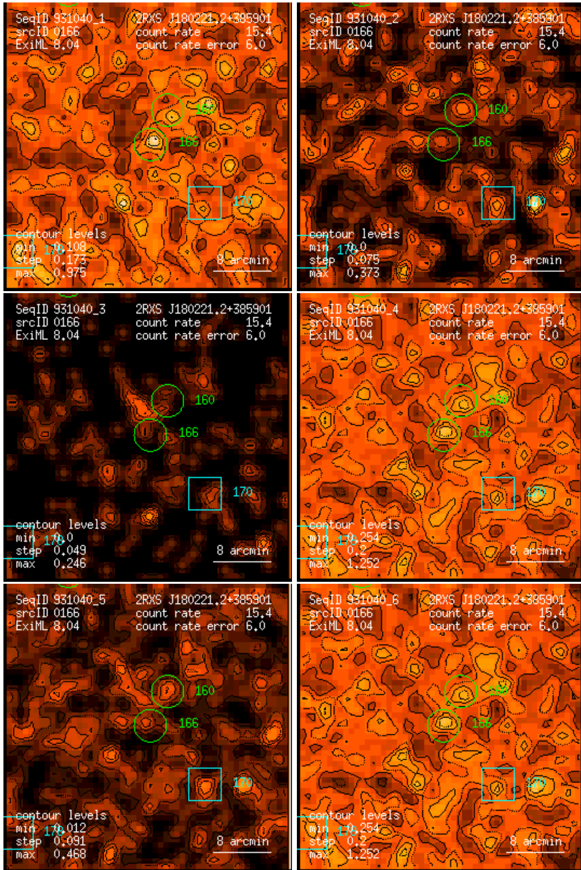
Figure 166: RASS 931040: detection 0166: band rate images, Gaussian filter: (1) PSPC channels 11 – 41, (2) 52 – 90, (3) 91 – 201, (4) 11 – 235, (5) 52 – 201, (6) 11 – 201. Broad band rates in counts/ks. Band rate contour levels in counts/ks/arcmin 2 .
