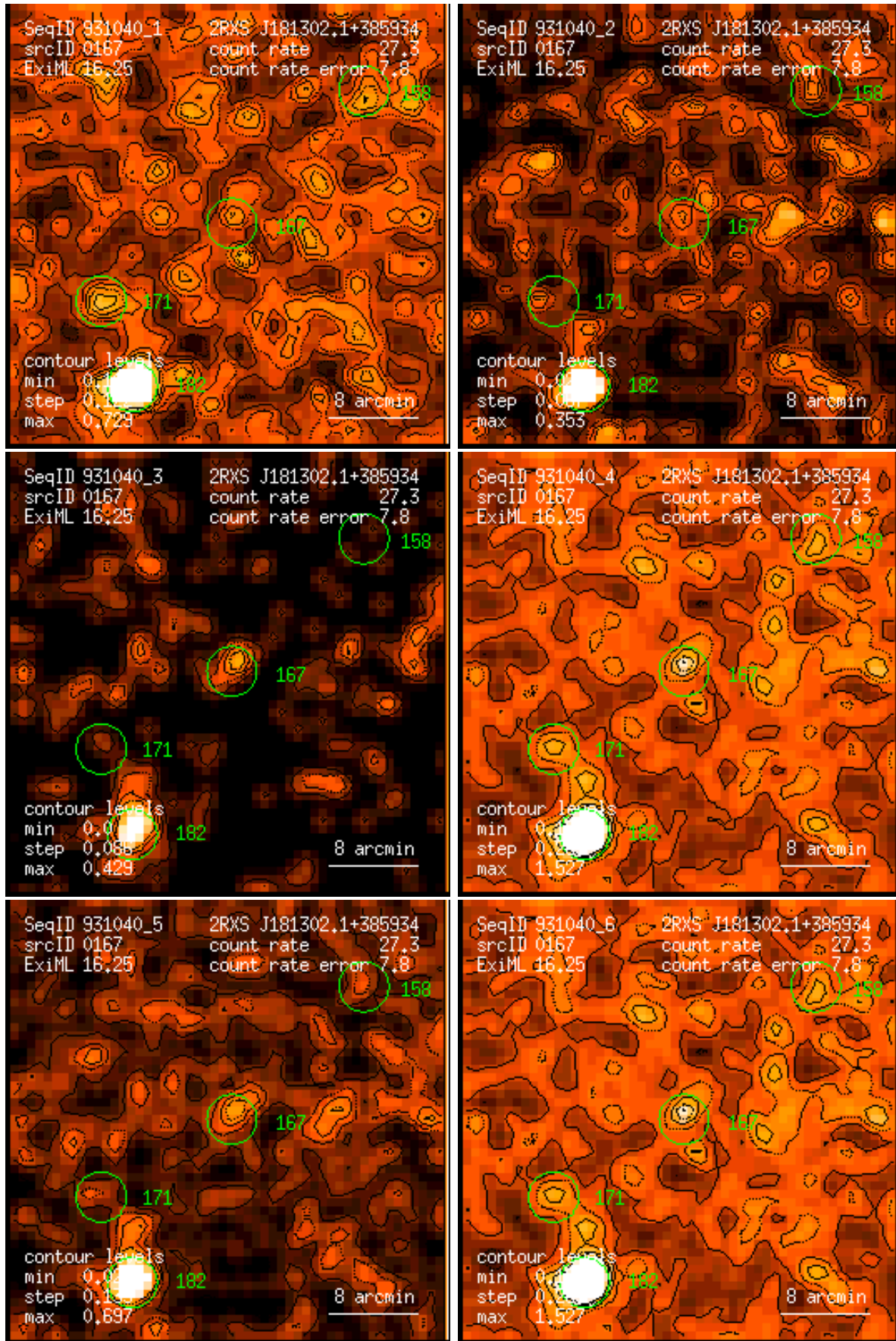
Figure 167: RASS 931040: detection 0167: band rate images, Gaussian filter: (1) PSPC channels 11 – 41, (2) 52 – 90, (3) 91 – 201, (4) 11 – 235, (5) 52 – 201, (6) 11 – 201. Broad band rates in counts/ks. Band rate contour levels in counts/ks/arcmin 2 .
