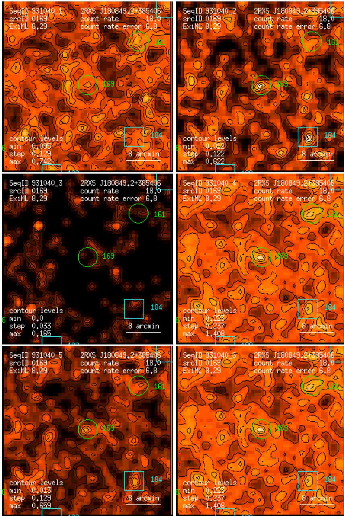
Figure 169: RASS 931040: detection 0169: band rate images, Gaussian filter: (1) PSPC channels 11 – 41, (2) 52 – 90, (3) 91 – 201, (4) 11 – 235, (5) 52 – 201, (6) 11 – 201. Broad band rates in counts/ks. Band rate contour levels in counts/ks/arcmin 2 .
