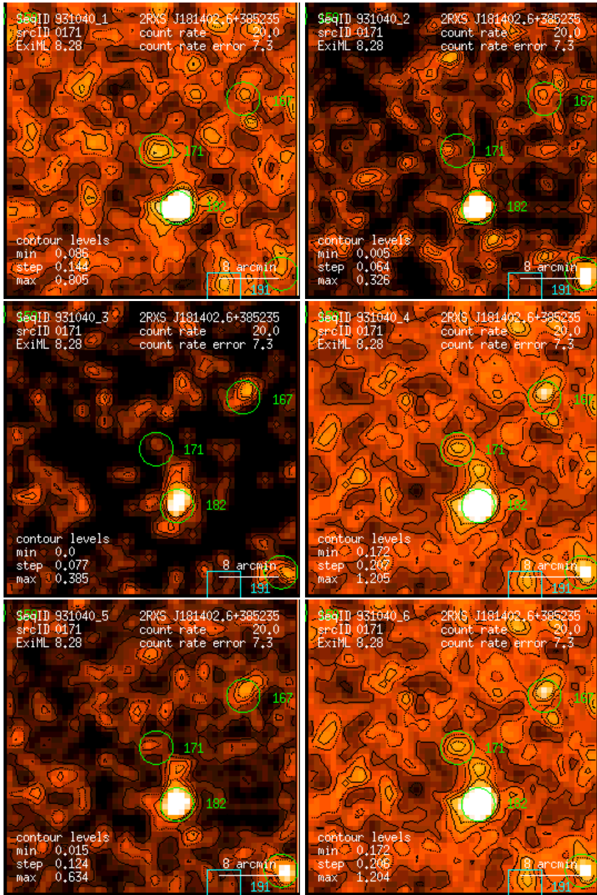
Figure 171: RASS 931040: detection 0171: band rate images, Gaussian filter: (1) PSPC channels 11 – 41, (2) 52 – 90, (3) 91 – 201, (4) 11 – 235, (5) 52 – 201, (6) 11 – 201. Broad band rates in counts/ks. Band rate contour levels in counts/ks/arcmin 2 .
