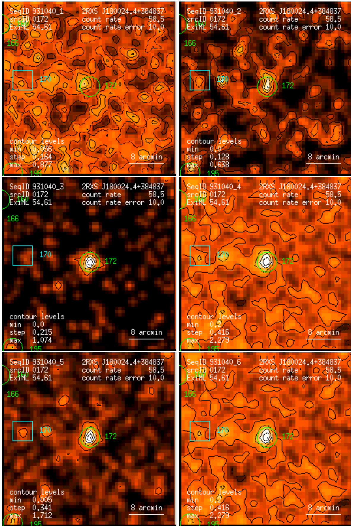
Figure 172: RASS 931040: detection 0172: band rate images, Gaussian filter: (1) PSPC channels 11 – 41, (2) 52 – 90, (3) 91 – 201, (4) 11 – 235, (5) 52 – 201, (6) 11 – 201. Broad band rates in counts/ks. Band rate contour levels in counts/ks/arcmin 2 .
