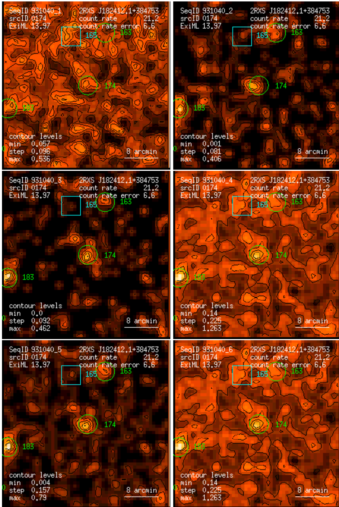
Figure 174: RASS 931040: detection 0174: band rate images, Gaussian filter: (1) PSPC channels 11 – 41, (2) 52 – 90, (3) 91 – 201, (4) 11 – 235, (5) 52 – 201, (6) 11 – 201. Broad band rates in counts/ks. Band rate contour levels in counts/ks/arcmin 2 .
