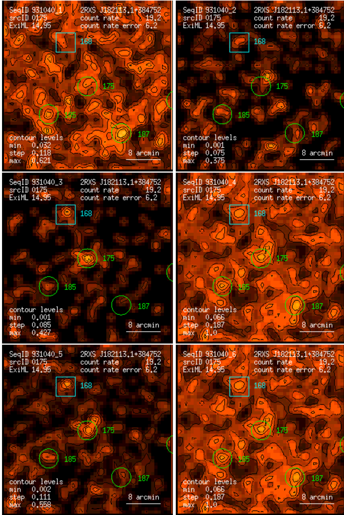
Figure 175: RASS 931040: detection 0175: band rate images, Gaussian filter: (1) PSPC channels 11 – 41, (2) 52 – 90, (3) 91 – 201, (4) 11 – 235, (5) 52 – 201, (6) 11 – 201. Broad band rates in counts/ks. Band rate contour levels in counts/ks/arcmin 2 .
