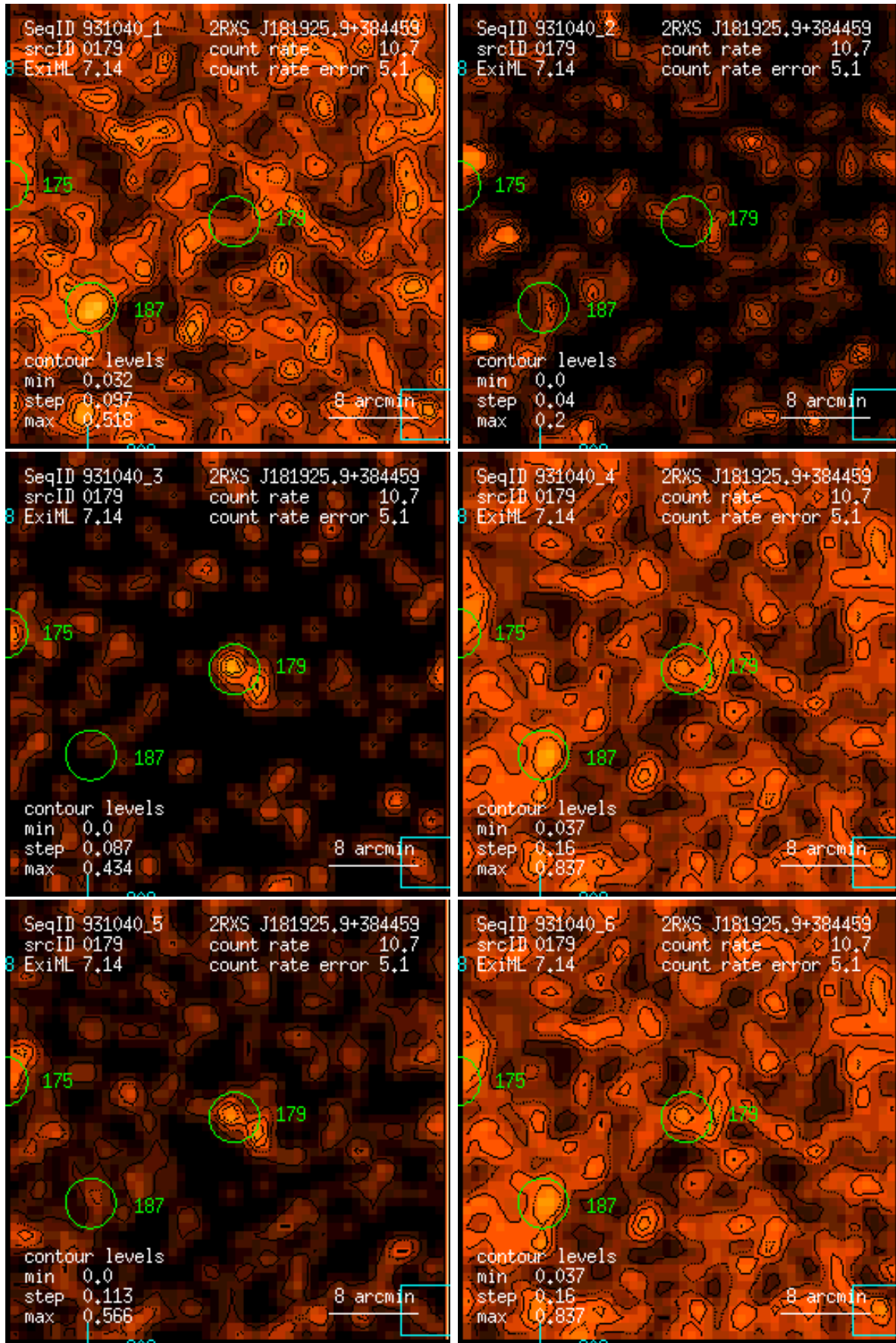
Figure 179: RASS 931040: detection 0179: band rate images, Gaussian filter: (1) PSPC channels 11 – 41, (2) 52 – 90, (3) 91 – 201, (4) 11 – 235, (5) 52 – 201, (6) 11 – 201. Broad band rates in counts/ks. Band rate contour levels in counts/ks/arcmin 2 .
