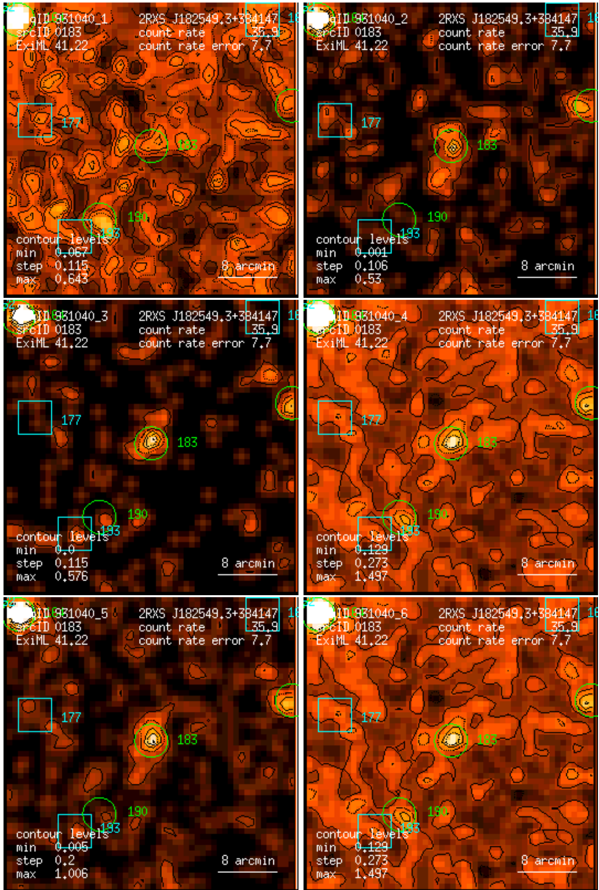
Figure 183: RASS 931040: detection 0183: band rate images, Gaussian filter: (1) PSPC channels 11 – 41, (2) 52 – 90, (3) 91 – 201, (4) 11 – 235, (5) 52 – 201, (6) 11 – 201. Broad band rates in counts/ks. Band rate contour levels in counts/ks/arcmin 2 .
