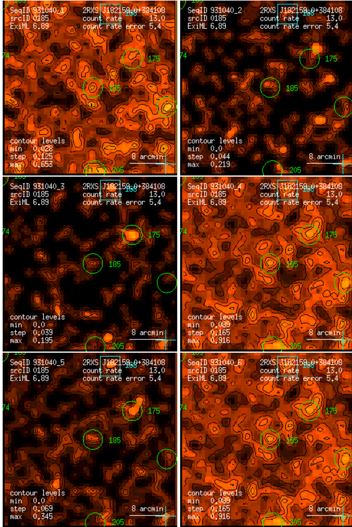
Figure 185: RASS 931040: detection 0185: band rate images, Gaussian filter: (1) PSPC channels 11 – 41, (2) 52 – 90, (3) 91 – 201, (4) 11 – 235, (5) 52 – 201, (6) 11 – 201. Broad band rates in counts/ks. Band rate contour levels in counts/ks/arcmin 2 .
