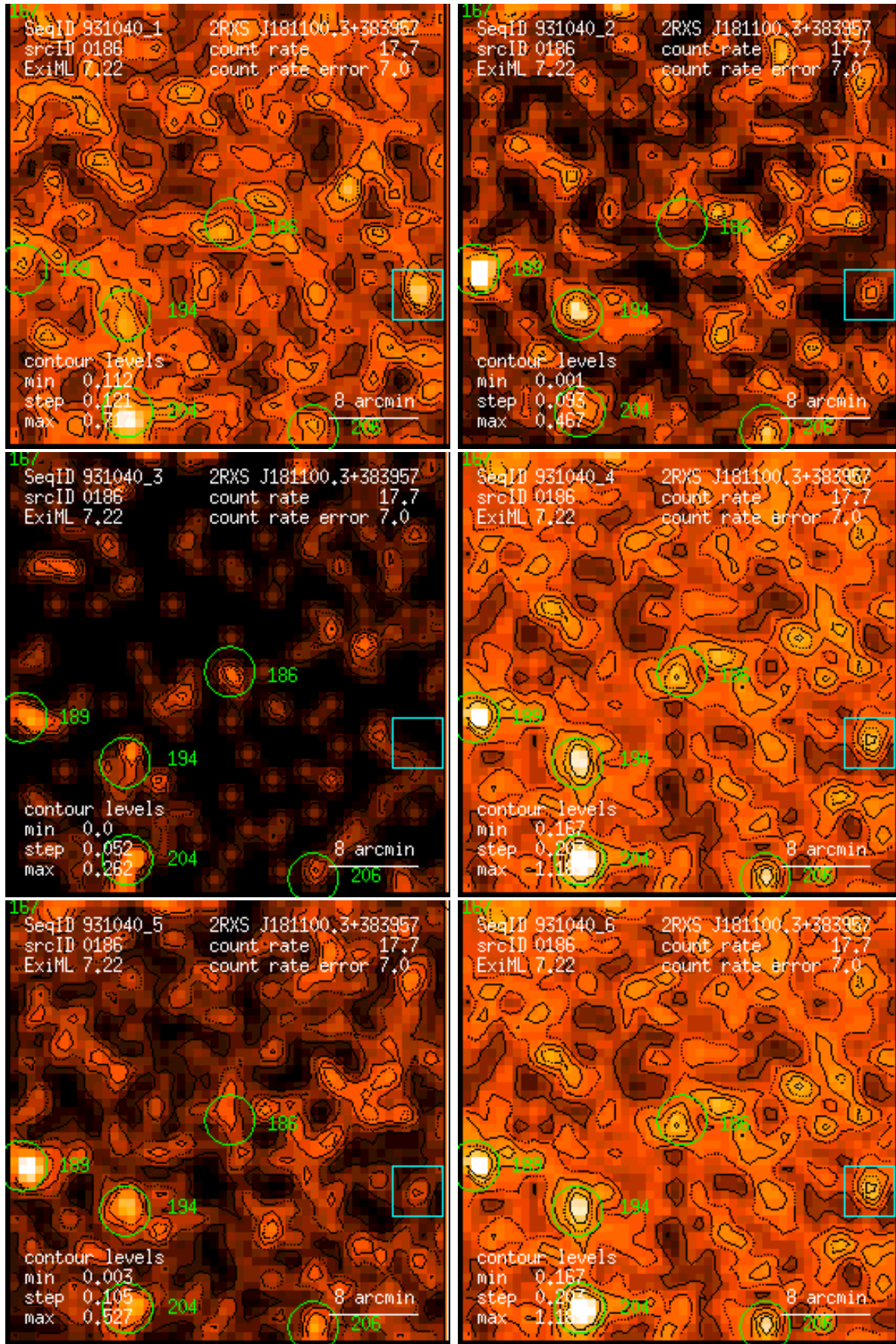
Figure 186: RASS 931040: detection 0186: band rate images, Gaussian filter: (1) PSPC channels 11 – 41, (2) 52 – 90, (3) 91 – 201, (4) 11 – 235, (5) 52 – 201, (6) 11 – 201. Broad band rates in counts/ks. Band rate contour levels in counts/ks/arcmin 2 .
