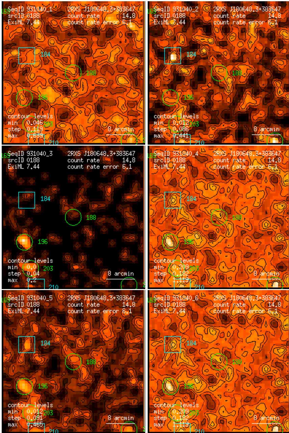
Figure 188: RASS 931040: detection 0188: band rate images, Gaussian filter: (1) PSPC channels 11 – 41, (2) 52 – 90, (3) 91 – 201, (4) 11 – 235, (5) 52 – 201, (6) 11 – 201. Broad band rates in counts/ks. Band rate contour levels in counts/ks/arcmin 2 .
